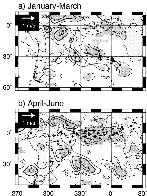
FIG. 7. Regression maps of NCEP-NCAR reanalysis 850-hPa winds (vectors) and 500-hPa omega (contours) with leading monthly PC of South Atlantic SST 1950–99. (a) JFM average, and (b) AMJ average. Only statistically significant vectors are plotted and shading denotes significant omega values; the 95% significance level corresponds to a correlation value of 0.28, which assumes 40 degrees of freedom. The contour interval is 0.2 \times 10^{-2} \text{ Pa s}^{-1} .
