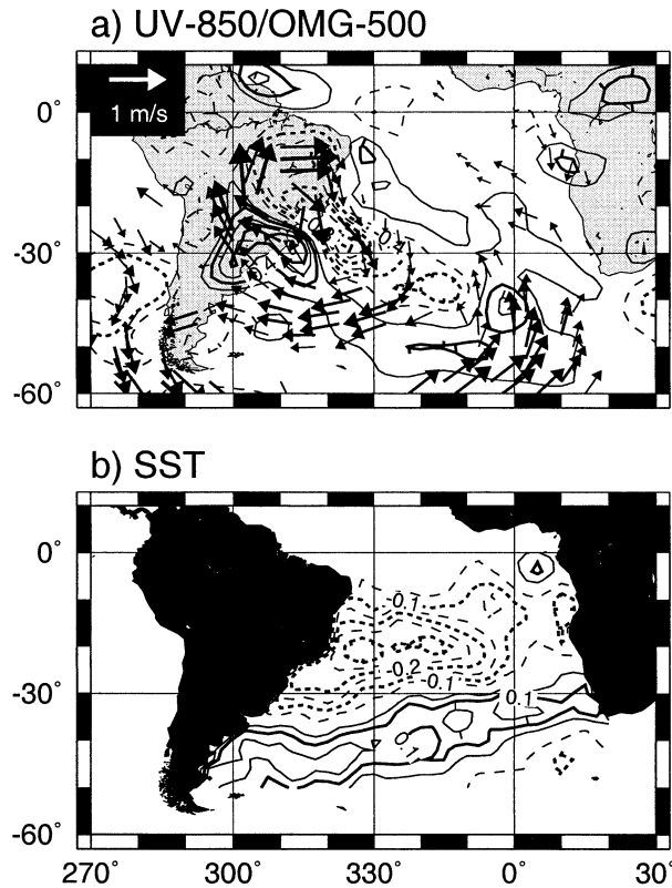
FIG. 1. Regression maps of the leading PC of 200-hPa JFM-averaged winds 1958–97 over southern South America from the NCEP–NCAR reanalysis. (a) 850-hPa winds and 500-hPa omega, (b) GISST SST. In (a), only vectors whose correlations with the PC are significant at the 95% level are plotted, with the number of degrees of freedom of the two-sided Student's t test estimated at each grid point from the decorrelation times of the PC and winds time series (Davis 1976). See Robertson and Mechoso (2000) for further details. Contour intervals are (a) 0.2 \times 10^{-2} \text{ Pa s}^{-1} , and (b) 0.05 K, with the zero contour omitted. Amplitudes correspond to a one std dev excursion of the PC.
