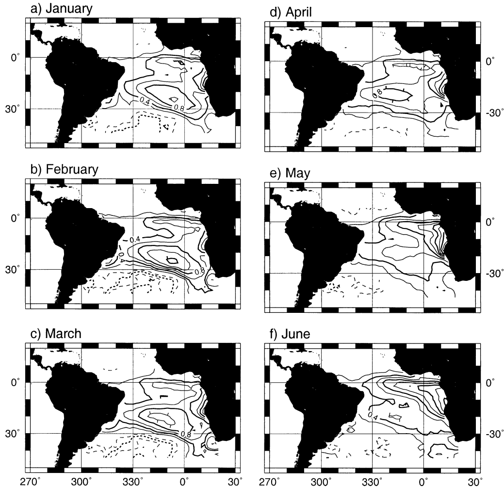
FIG. 4. Seasonal evolution of SST anomalies used to force the GCM in the experiment described in section 4. See text for details. Contour interval is 0.2 K, with the zero contour omitted.
