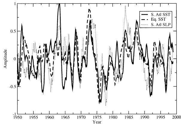
FIG. 10. Twelve-month running average anomaly time series of (a) subtropical South Atlantic SST ( 14^{\circ} – 26^{\circ} S, 20^{\circ} W– 0^{\circ} ; solid line), (b) equatorial SST ( 2^{\circ} N– 4^{\circ} S, 10^{\circ} W– 0^{\circ} ; dashed line), and (c) normalized SLP ( 15^{\circ} – 45^{\circ} S, 30^{\circ} W– 0^{\circ} ; thin dotted line) multiplied by -1 . The units of SST are K.
