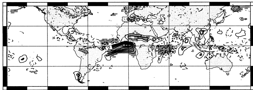
FIG. 8. Global AMJ response to the SST anomaly evolution in Fig. 4. (a) 200-hPa winds and streamfunction (contour interval 1.5 \times 10^{-6} \text{ m}^2 \text{ s}^{-1} , zero contour included), (b) precipitation (contour interval 0.5 \text{ mm day}^{-1} , zero contour omitted). Other details as in Fig. 6.
