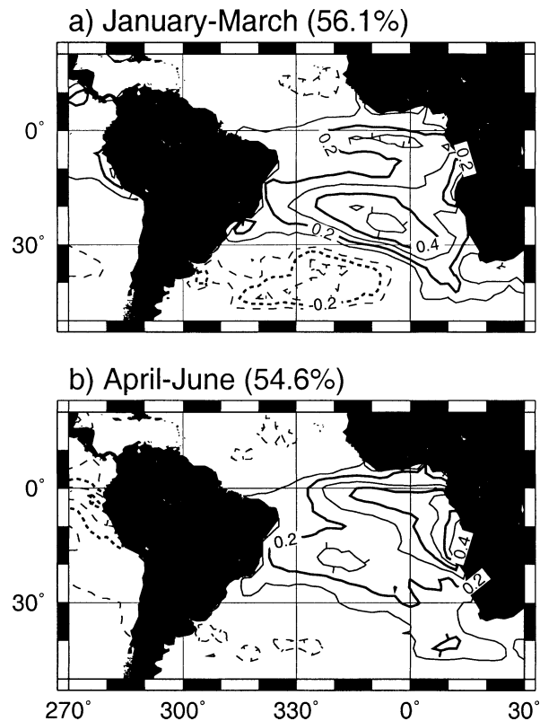
FIG. 3. The leading seasonal-mean EOF of the (linearly detrended) Reynolds SST dataset 1950–99, computed over the South Atlantic 0°–30°S for (a) JFM, and (b) AMJ. Shown are regression maps with the respective PC. Contour interval is 0.1 K, with the zero contour omitted.
