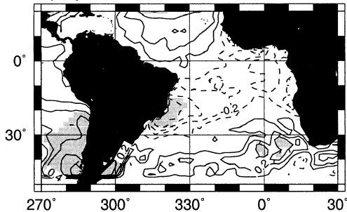
FIG. 9. Correlation maps of seasonal mean Reynolds SST with the JFM PC used to construct Fig. 1. (a) Preceding Oct-Feb, (b) contemporaneous JFM, and (c) the following AMJ. Locally 95% significant areas are shaded, as in Fig. 1. Contour interval is 0.1, with zero contour omitted.
