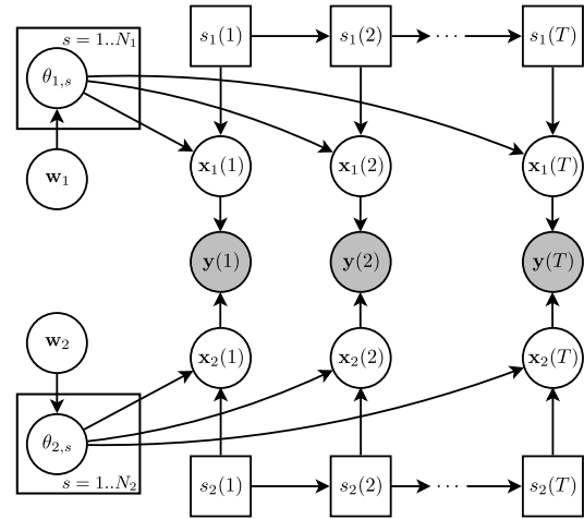
Fig. 1. Proposed mixed signal model. The mixture observations \mathbf{y}(t) are explained as the combination of two hidden source signals \mathbf{x}_1(t) and \mathbf{x}_2(t) . Each source signal is modelled by a separate speaker-adapted hidden Markov model, that is derived from the speaker subspace model described in section 2.
