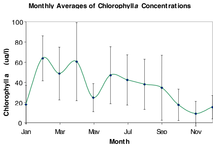
Figure 7.9-4: Monthly averages of chlorophyll \alpha concentration in Jamaica Bay, showing seasonal trends in production. Chlorophyll \alpha levels range from 8.90 g/l to 63.69 g/l with peaks in February through April, and June through August.
