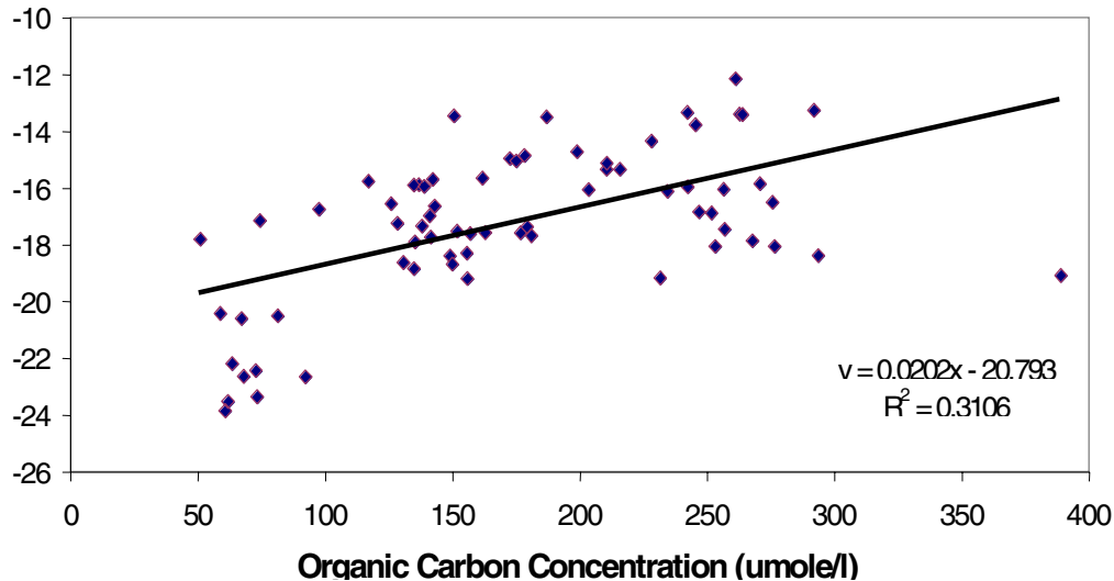
Figure 7.9-8: The relationship between organic carbon concentration and carbon isotopic composition ( \delta^{13}\text{C} ) in surface waters. \delta^{13}\text{C} values range from -23.86 to -12.16 . Carbon concentration ranges from 51.10 to 389.09 mole/l. A positive correlation exists between the two variables with an R^2 value of 0.3106 . Note that the \delta^{13}\text{C} of inorganic carbon in the atmosphere is between -7.0 and -8.0 .
