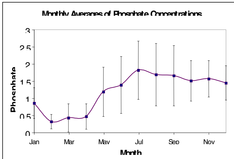
Figure 7.9-3: The monthly averages for phosphate concentration in Jamaica Bay, showing seasonal trends in nutrient levels. Phosphate levels range from 0.32 mole/l to 1.82 mole/l with high levels in May through November.
