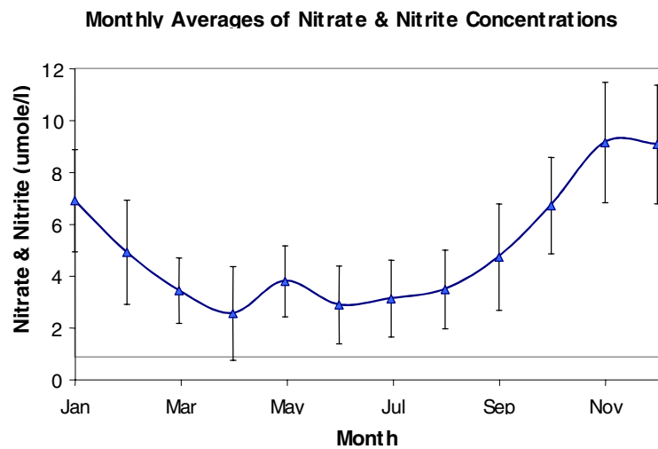
Figure 7.9-2: Monthly averages for nitrate and nitrite concentrations in Jamaica Bay, show seasonal trends in nutrient levels. Nitrate and nitrite levels range from 2.55 mole/l to 9.14 mole/l with peaks in May and November through January.
