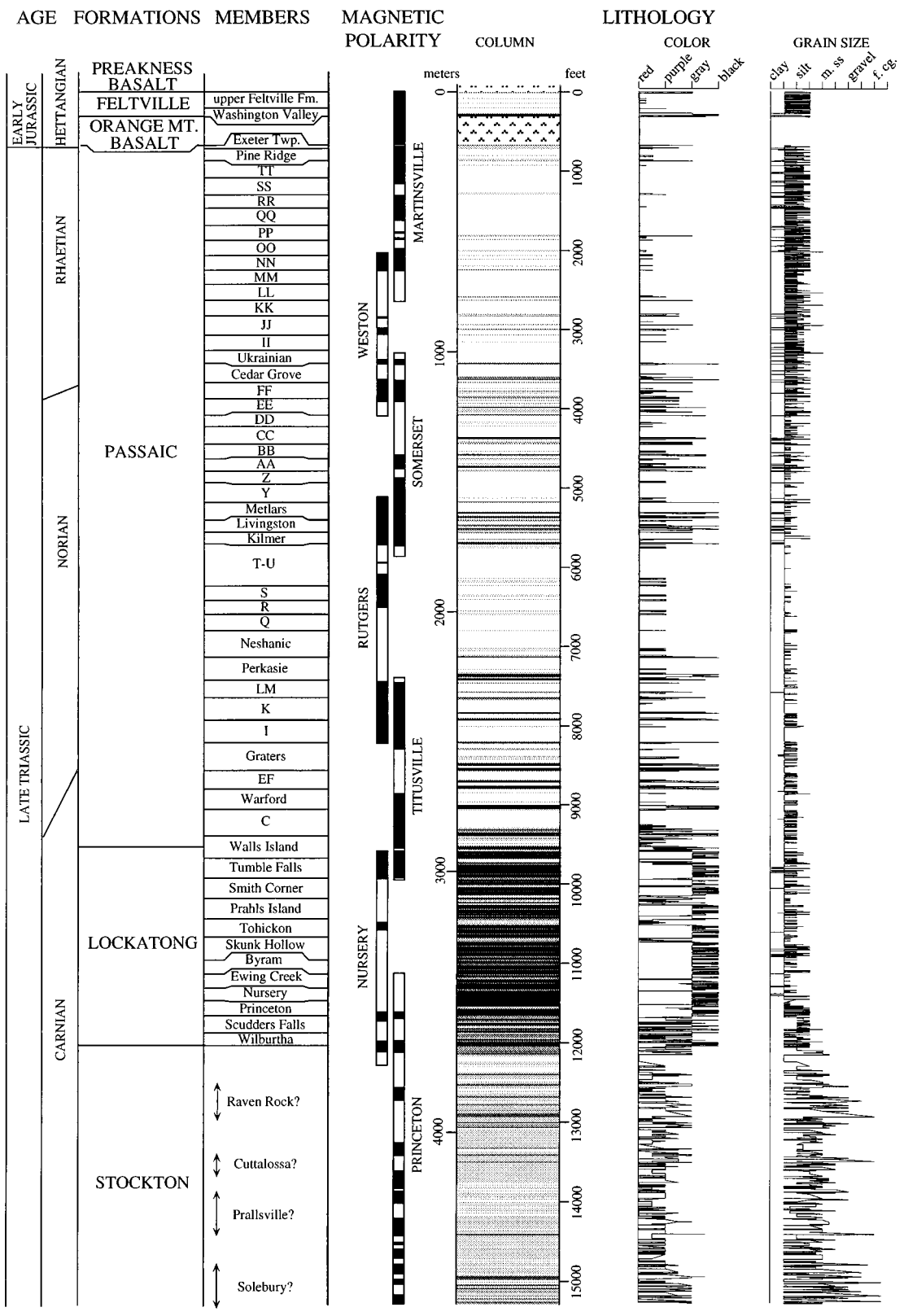
Figure 30. Composite section of Newark Basin Coring Project Cores. All cores have been scaled to the Rutgers no. 1 and 2 cores.
