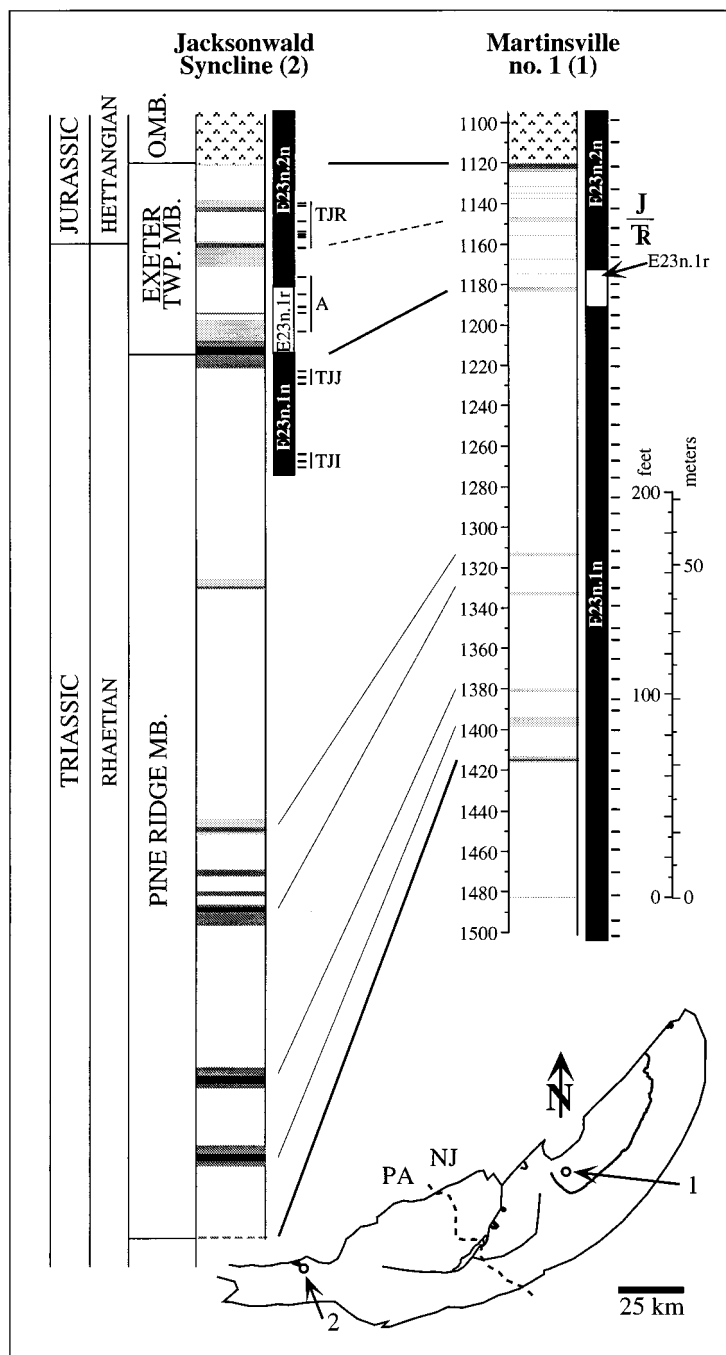
Figure 27. Correlation of the uppermost Passaic Formation in the Martinsville no. 1 core (1) with the type sections of the Pine Ridge and Exeter Township members and the paleontologically identified Triassic-Jurassic boundary in the Jacksonwald syncline. Lithologic and paleomagnetic key as in Figure 13, and other abbreviations and symbols as follows: TJR, TJJ, TJI, symbols for sampling sites in Witte et al. (1991); A, samples processed for this work; horizontal ticks, sample sites. Upper part of section (to base of paleomagnetic samples) is based on exposures along Sycamore Drive, Exeter Township, Berks County, Pennsylvania, and the adjacent type section of the Exeter Township Member. Lower part of the section for Jacksonwald Syncline (below paleomagnetic samples) is based on temporary exposures along Constitution and Pennsylvania avenues, Exeter Township, Berks County, Pennsylvania, and type exposures of Pine Ridge Member along nearby creek. PA, Pennsylvania; NJ, New Jersey; O.M.B., Orange Mountain Basalt.
