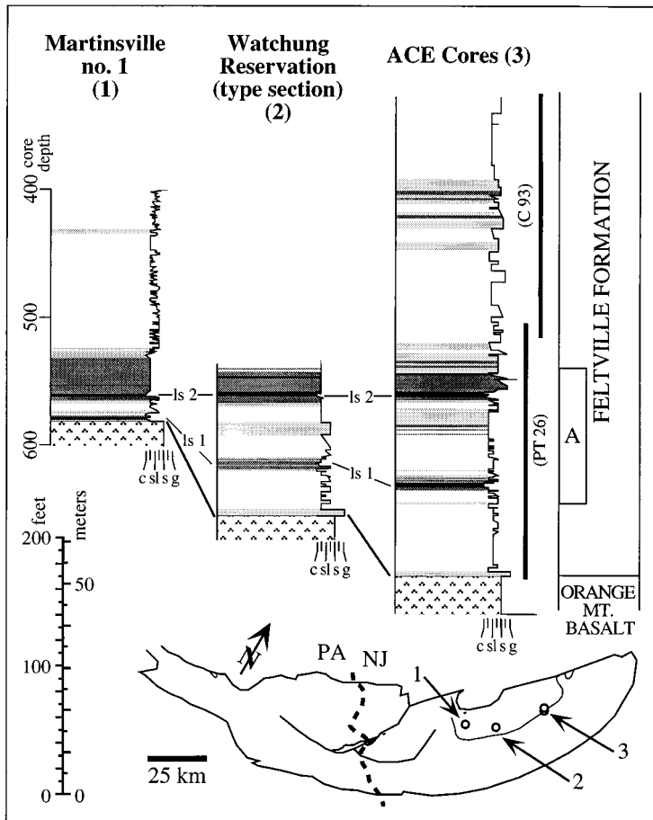
Figure 28. Comparison of the type section of Feltville Formation in Watchung Reservation (2), Martinsville no. 1 (1), and ACE cores (cores PT-26 and C-93) (3). A, interval designated the informal Washington Valley member. PA, Pennsylvania; NJ, New Jersey; c, claystone; sl, siltstone; s, sandstone; g, gravel; ls, limestone.
