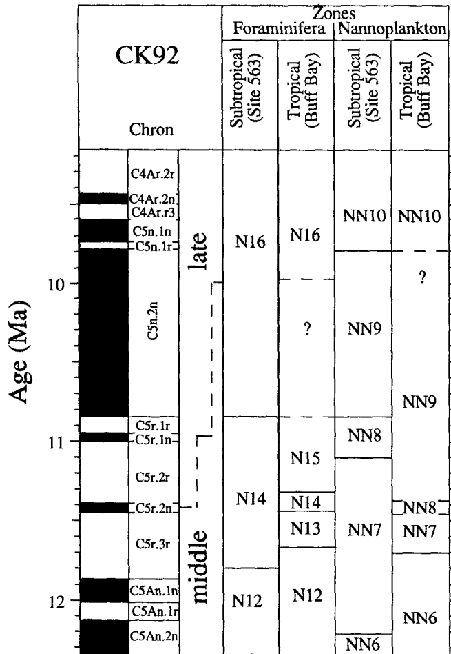
Figure 4. Revised late middle to early late Miocene time scale showing the geomagnetic polarity time scale of Cande and Kent (1992), ages of subtropical zones developed at Site 563 (Table B), and tropical zones developed using Buff Bay calibrations. The middle/late Miocene boundary is placed within Zone NN8 immediately before the FO of N. acostaensis (= base of Zone N16). The placement of the base of tropical Zone N16 is uncertain and is higher than subtropical Zone N16 based on relationships at Site 289.
