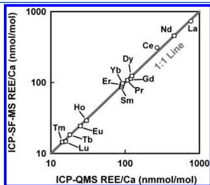
Figure 5. Comparison of measured REE/Ca ratios of a benthic foraminifer, C. wuellerstorfi , from marine core MW91-9 GGC-15 by our ICP-SF-MS and ICP-QMS 27,28 at the University of Cambridge.
