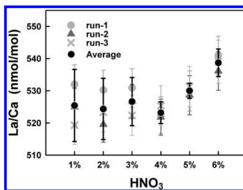
Figure 2. Acid effect of \text{HNO}_3 , 1–6%, on La/Ca measurement for the CarbREE-I standard solution with a constant Ca concentration of 20 ppm. Three duplicates are shown in gray symbols with internal errors. The averages are shown in solid circles with 2\sigma .
