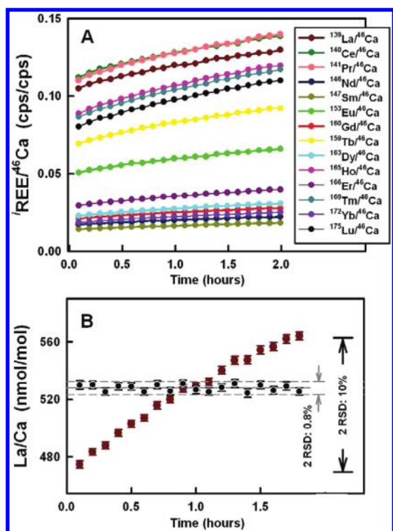
Figure 1. (A) Mass drifting in measured REE isotope ( i\text{REE} )/ ^{46}\text{Ca} ratios over a 2 h analysis for the 20 ppm Ca CarbREE-I standard solution. (B) Ratio drift in La/Ca over a 2 h measurement experiment. Short-term 2 RSD external precision is improved from \pm 10\% (dark red circles) for the uncorrected values to \pm 0.8\% (black circles) for the standard-bracketing corrected data.
