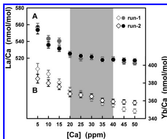
Figure 3. Repeat runs for Ca concentration effect on determinations of (A) La/Ca and (B) Yb/Ca. There is a minor [Ca] effect between 20 and 40 ppm (shaded area) (see text).
