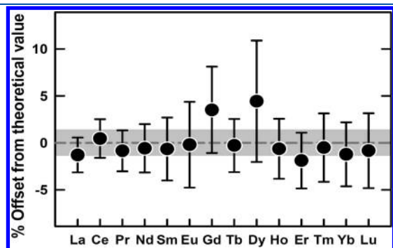
Figure 4. Percent offset of measured REE/Ca ratios with long-term 2 RSD error bars (Table S4) from theoretical values in the CoralM-REE standard solution. The shaded area denotes the uncertainty of REE/Ca in the standard.
