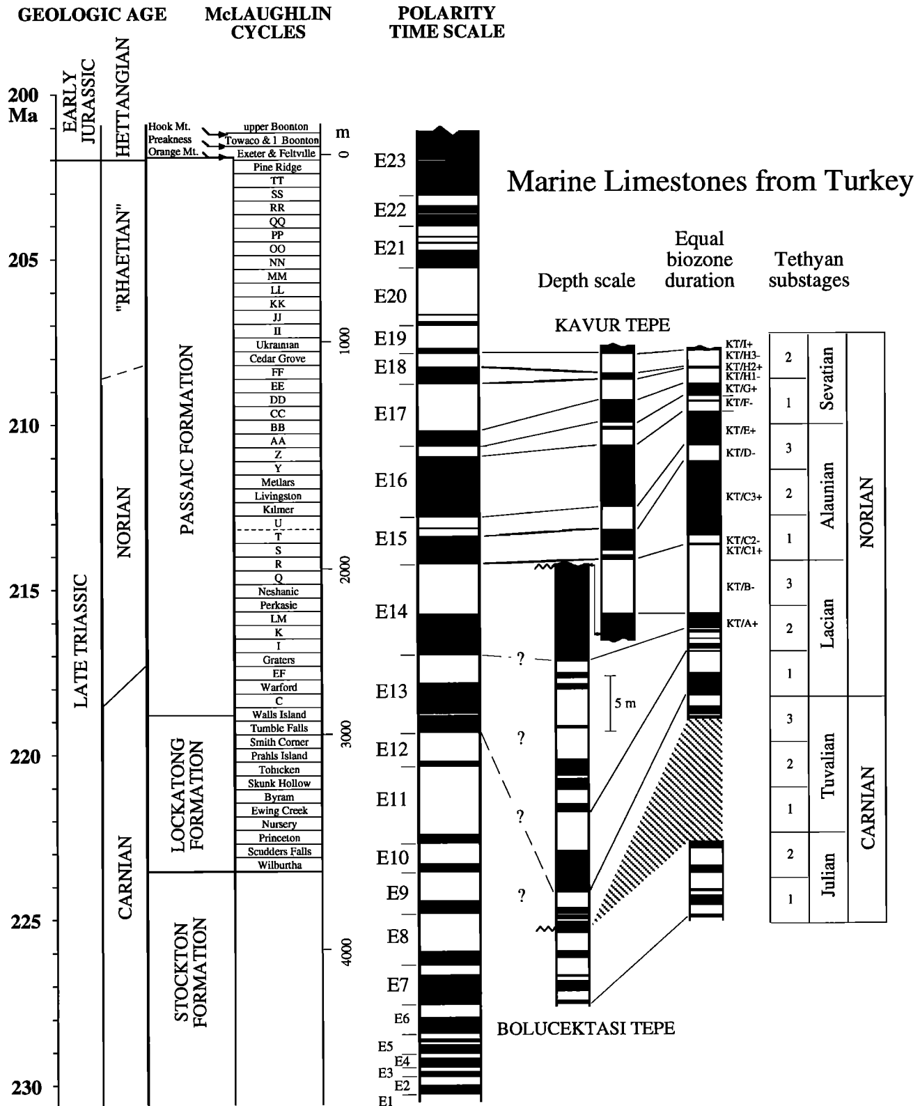
Figure 22. Magnetostratigraphies from marine limestone sections from Turkey (Bölüçektasi Tepe [Gallet et al., 1992] and Kavur Tepe [Gallet et al., 1993]) with possible correlations to the Newark geomagnetic polarity timescale. Subdivisions of the Norian and Carnian are plotted on a linear timescale with arbitrary scale assuming equal duration of the Tethyan (sub)substages; magnetostratigraphies of the limestone sections are shown in terms of measured thickness (see scale) and as transformed in a composite to an equal biozone duration timescale on the basis of conodont biostratigraphy [Gallet et al., 1992, 1993]. The upper third of the Bölüçektasi Tepe section, which includes an approximately 25-m-thick normal polarity interval which was correlated to the KT/C3+ magnetozone in Kavur Tepe [Gallet et al., 1993], has been omitted for clarity.
