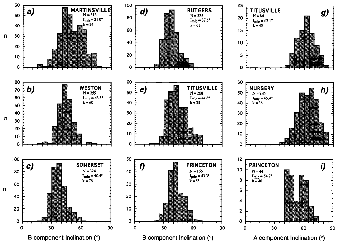
Figure 6. Inclinations of overprint magnetizations ((a)-(f) B component; (g)-(i) A component) isolated in samples from NBCP drill cores. Maximum likelihood estimates for mean inclination ( I_{mle} ) and precision parameter ( k ) calculated using technique of McFadden and Reid [1982; corrected algorithm from Schneider , 1989] on inclinations with respect to present horizontal (i.e., drill cores corrected only for hole deviation). Expected inclination for B component is 42^\circ [Witte and Kent, 1991] and for A component is dipole field local value of 59^\circ .
