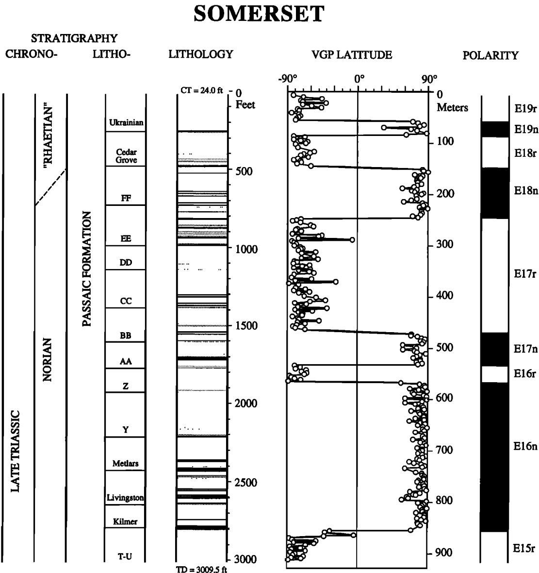
Figure 13. Physical stratigraphy, lithology, and magnetostratigraphy of the Somerset drill core. Conventions as in Figure 9.
