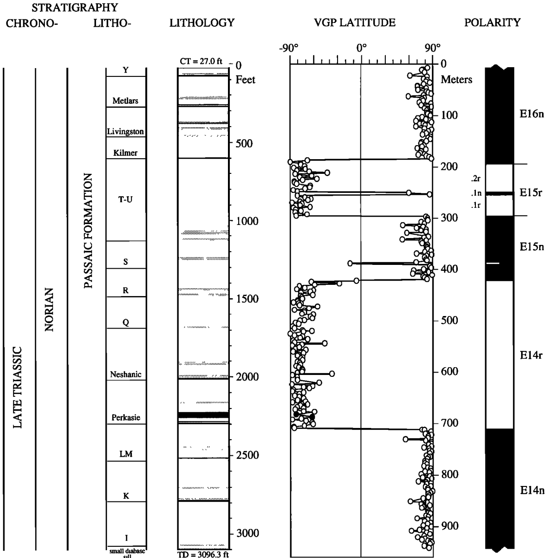
Figure 12. Physical stratigraphy, lithology, and magnetostratigraphy of the Rutgers drill core. Conventions as in Figure 9.
