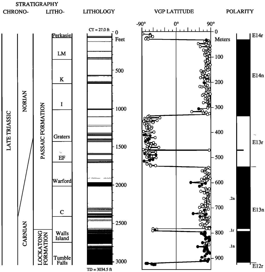
Figure 11. Physical stratigraphy, lithology, and magnetostratigraphy of the Titusville drill core. Conventions as in Figure 9.
