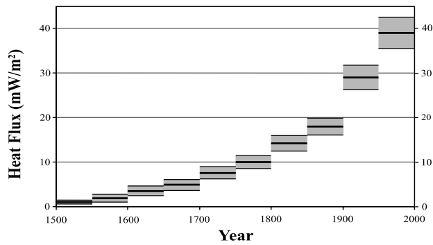
Figure 2. Global heat flux history inferred from the global average GSTH determined from subsurface temperature inversions. The mean heat flux over fifty-year intervals is shown as heavy black lines. The gray shaded areas represent the uncertainty about the means.
