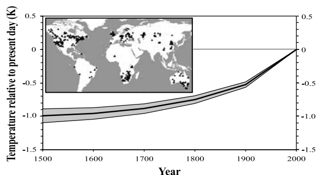
Figure 1. Global average of GSTH over the past five centuries. Shaded areas represent \pm 1 standard error about the mean. Inset shows the location of the 616 boreholes where subsurface temperature measurements have been analyzed to reconstruct the global GSTH.
