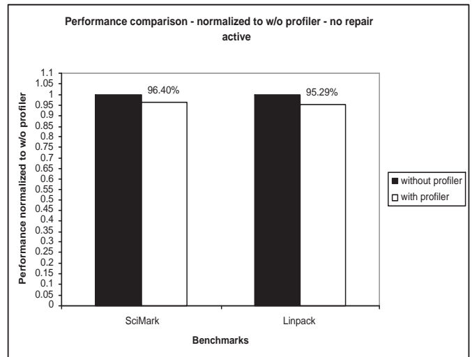
Figure 7: Overheads when no repair active
