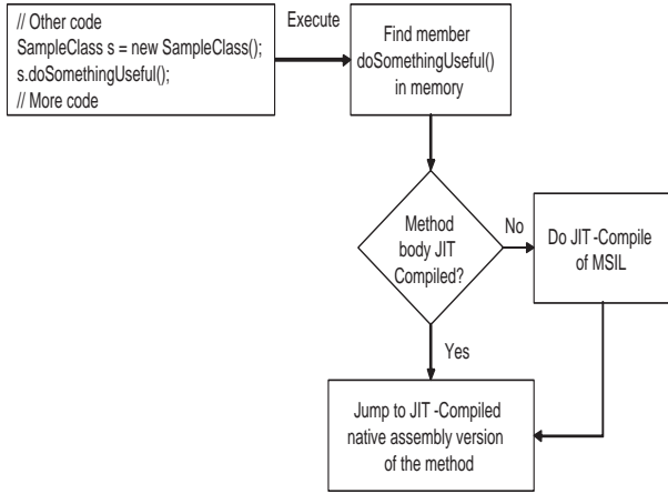
Figure 1: Overview of the CLR execution cycle
