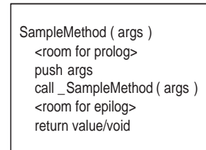
Figure 6: Conceptual diagram of a Wrapper
