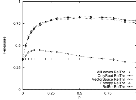
Figure 4: Average F -measure for the link-based strategy of Section 3 as a function of p ( RelThr pruning strategy).
