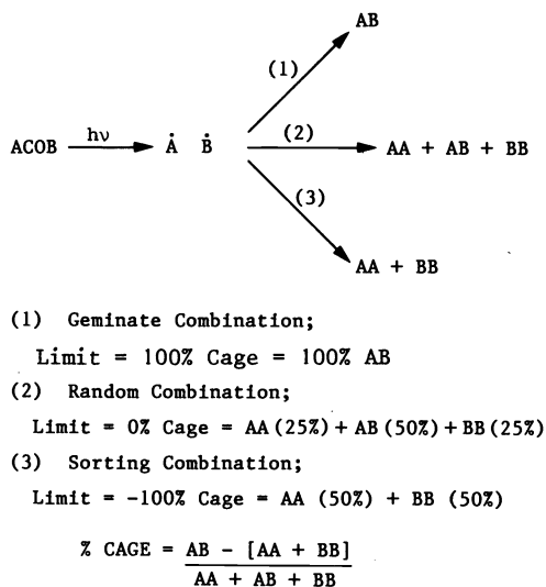
Figure 8. General scheme for possible combinations of radical pairs.
