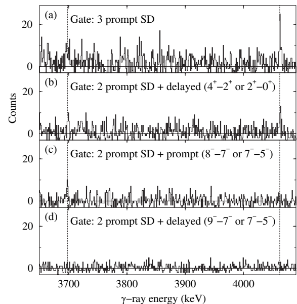
FIG. 2. Spectra showing the candidate SD-ND linking transitions. The gating conditions are indicated in the figure.
