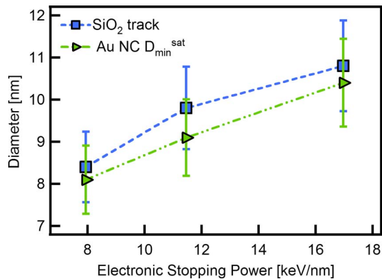
FIG. 3. (Color online) Saturation width of the irradiated Au NPs D_{\min}^{\text{sat}} and ion track diameter (see Ref. 13) as a function of electronic stopping power in SiO 2 .
