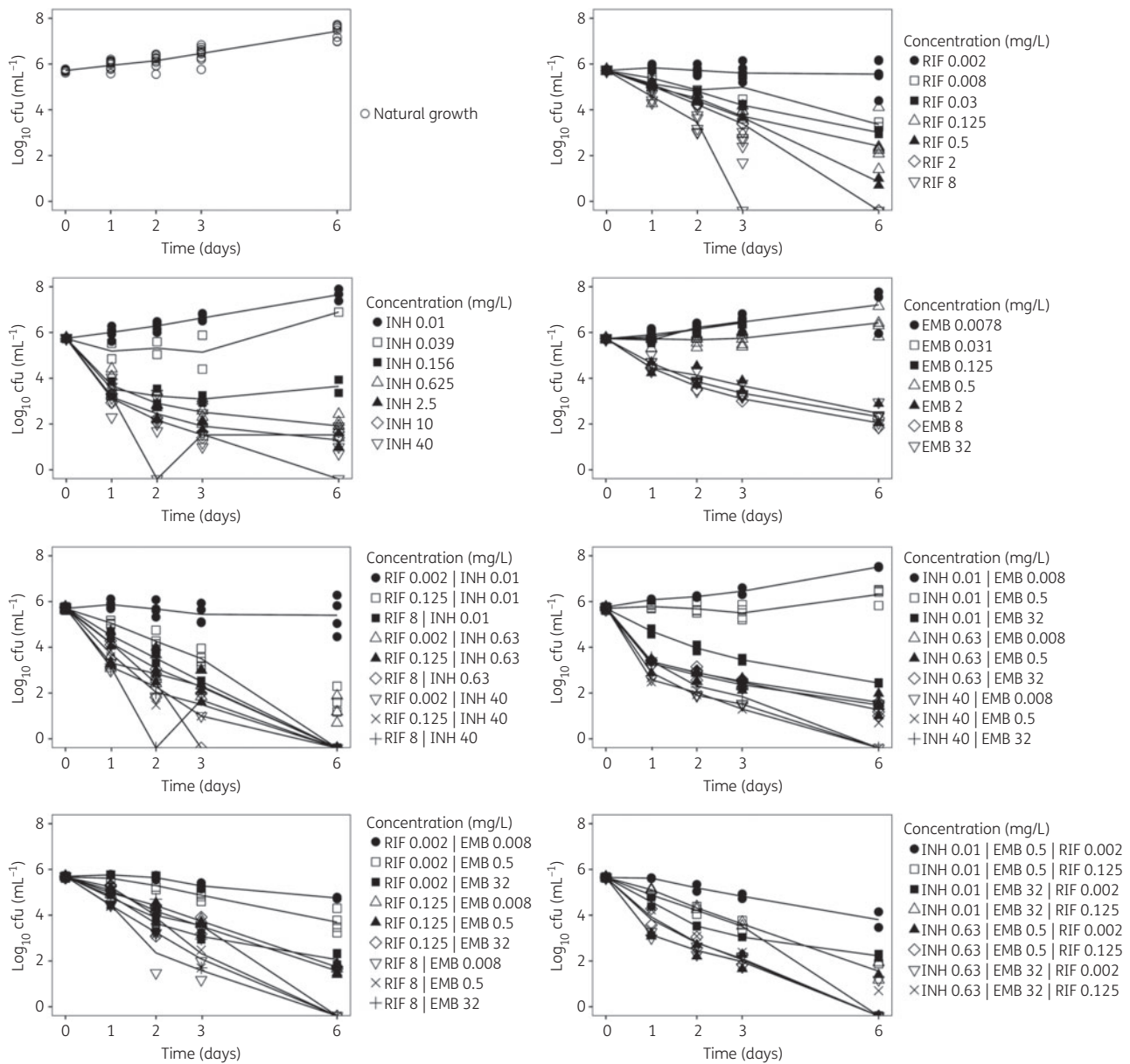
Figure 1. Mean observed log 10 cfu versus time for natural growth and time-kill curve studies with rifampicin (RIF), isoniazid (INH) and ethambutol (EMB) at different concentrations.
