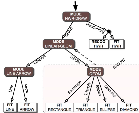
Figure 2. A hierarchical classification system for pen gestures. This system consists of three feature classifiers and one shape matching classifier. After classification takes place, a fit of the gestures to template objects may be performed.
