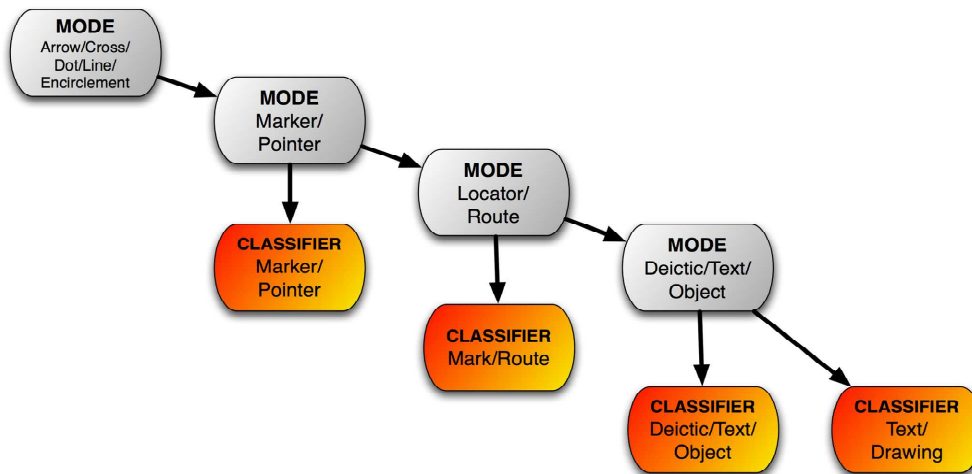
Figure 4. The Bayesian belief network used to combine the results of four different classifiers.
