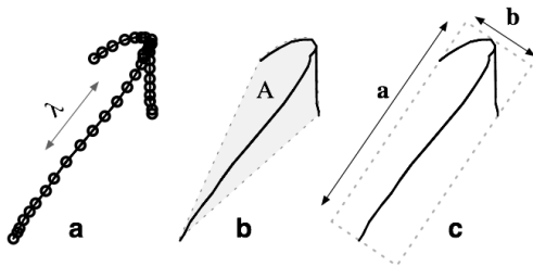
Figure 1. Examples of geometric features: (a) The length ( \lambda ) of the pen trajectory. (b) The area ( A ) of the convex hull of a pen trajectory. (c) The ratio of the principle axis of the bounding box ( a/b ).
