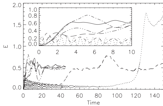
FIG. 1. Time history of the energy for set A: A1 (solid), A2 (dashed-dotted), A3 (dashed-triple dot), A4 (long dashed), A5 (dashed), and A6 (dotted); Rossby numbers range from 4.50 to 0.03. The inset shows a detail of the evolution at early times: At high rotation rates (runs A5 and A6), waves prevail and the energy of the system is lower than when little rotation is present. Note the transition to a high energy regime at later times as Ro decreases, because of an inverse energy cascade setting in (run A6 continues until t \approx 185 , while the energy keeps growing steadily).
