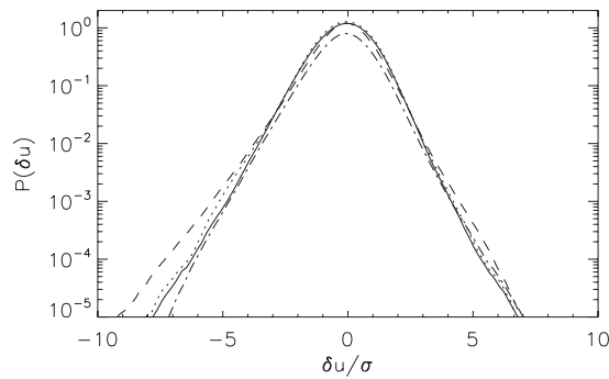
FIG. 14. pdf of the longitudinal velocity increments ( \ell_{\perp} = 3\eta ) for run B3 at different times: t \approx 20 (solid), t \approx 25 (dotted), t \approx 30 (dashed), and t \approx 40 (dashed-dotted); \eta is the Kolmogorov dissipative length and \sigma is the root mean square deviation of the velocity increments.
