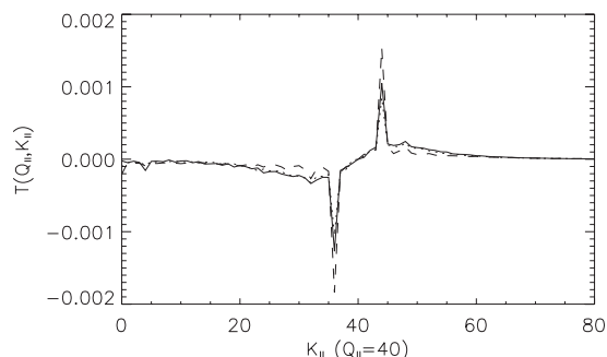
FIG. 10. Shell-to-shell transfer function T(Q_{\parallel}, K_{\parallel}) at Q_{\parallel}=40 for runs B1, B2, and B3. Labels are as in Fig. 8. Notice these transfers are roughly five times weaker than in the \perp case.
