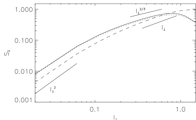
FIG. 12. Second order longitudinal structure function S_2(\ell_{\perp}) (where \ell_{\perp} denotes increments were taken in the direction perpendicular to \boldsymbol{\Omega} ) for runs B1 (solid), B2 (dotted), and B3 (dashed).
