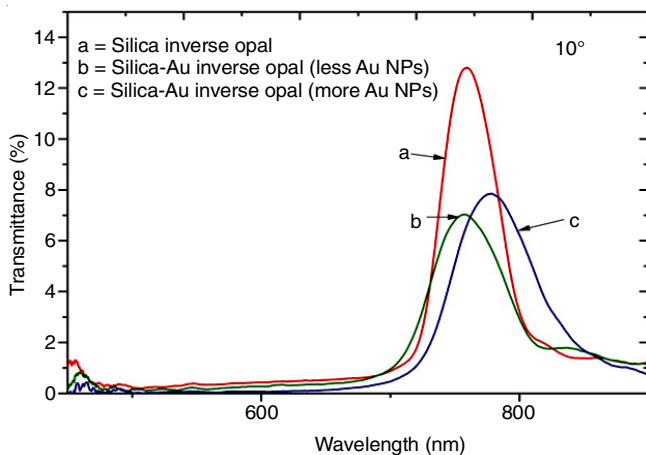
Fig. 4. Transmission spectra of inverted thin film and inverted MPDC thin film with two different gold nanoparticles percentage incorporated
