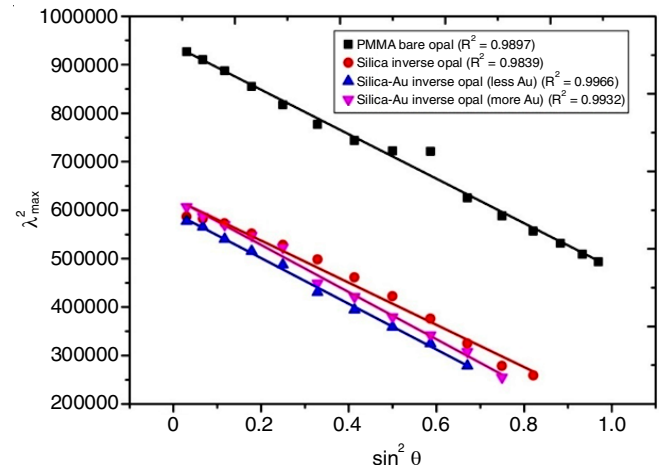
Fig. 5. Graph of \lambda_{max}^2 versus \sin^2\theta for PMMA bare opal, inverted structure and inverted MPDC thin film. This data was applied with a degree of departure from the Bragg-Snell's law
