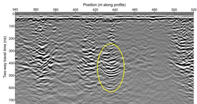
Fig. 4. Detail from Beacon Valley profile migrated at 0.120 m/ns. Note the stacked “smiles” (circled) at about 435 m along the profile.
