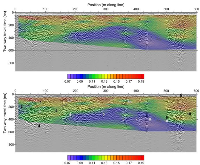
Fig. 5. Unmigrated merged (top) and migrated merged (bottom) profiles from 0 to 600 m, overlain by velocity variations.
