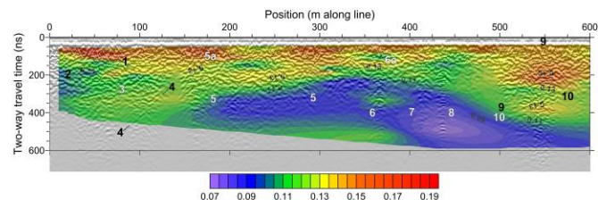
Fig. 6. Detail from Beacon Valley envelope profile. Note how many of the velocity boundaries correspond with strong reflection amplitudes.
