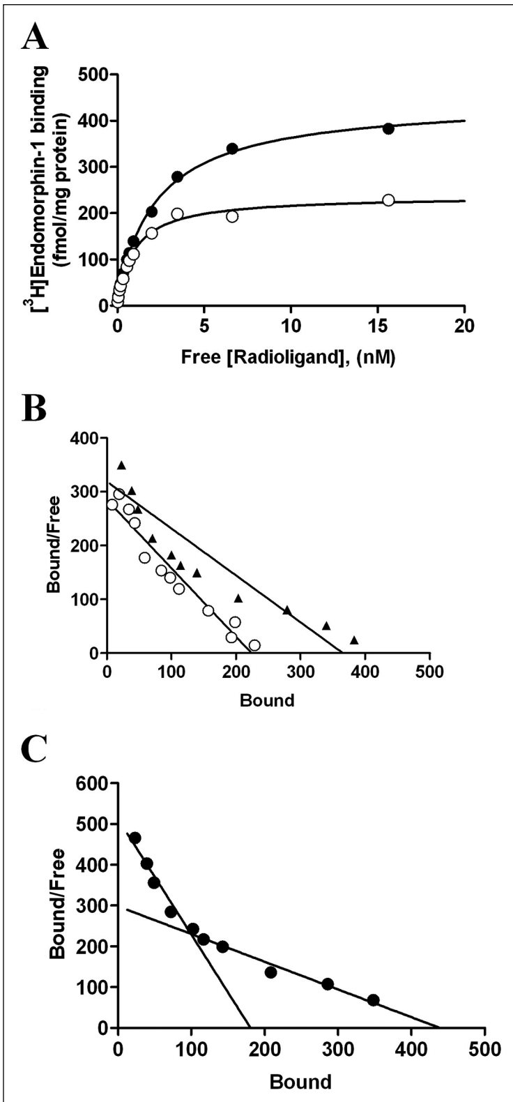
Fig. 1. Saturation binding curve and Scatchard plot of ^{3}\text{H} endomorfin-1 binding.
