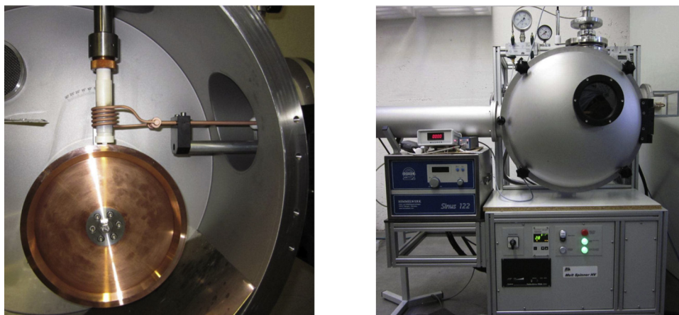
Fig. 1. Melt Spinner used in this work and its peripherals.
