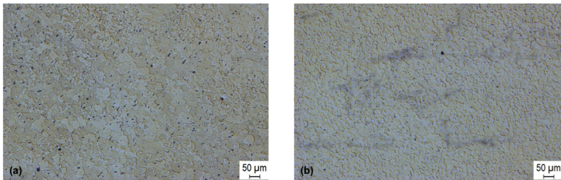
Fig. 6. Optical micrographs show addition of nickel resulted in grain refinement of melt spun ribbon; (a) base alloy and (b) base alloy plus ~3 wt.% Ni.
