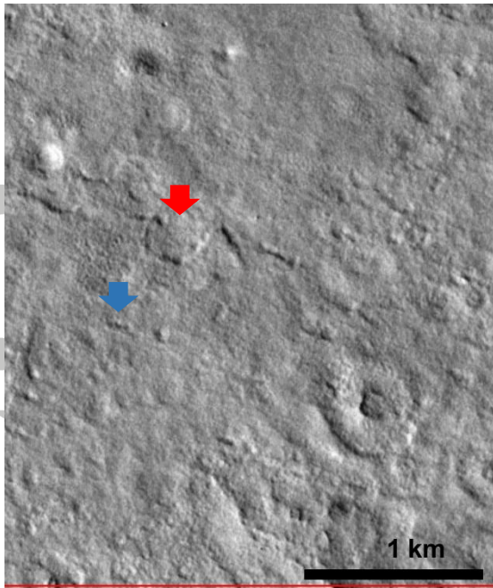
Figure 8 CTX image G03_019221_2327 showing the morphology of scalloped terrain (e.g. red arrow – i.e. not to be confused with pitted terrain e.g. blue arrow) in Arcadia Planitia.
