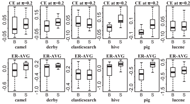
(a) B vs S evaluation under across-version change-proneness prediction with respect to api.
