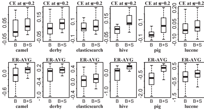
(b) B vs B+S evaluation under across-version change-proneness prediction with respect to api.
