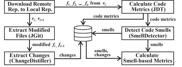
Fig. 1: Procedure of data collection
