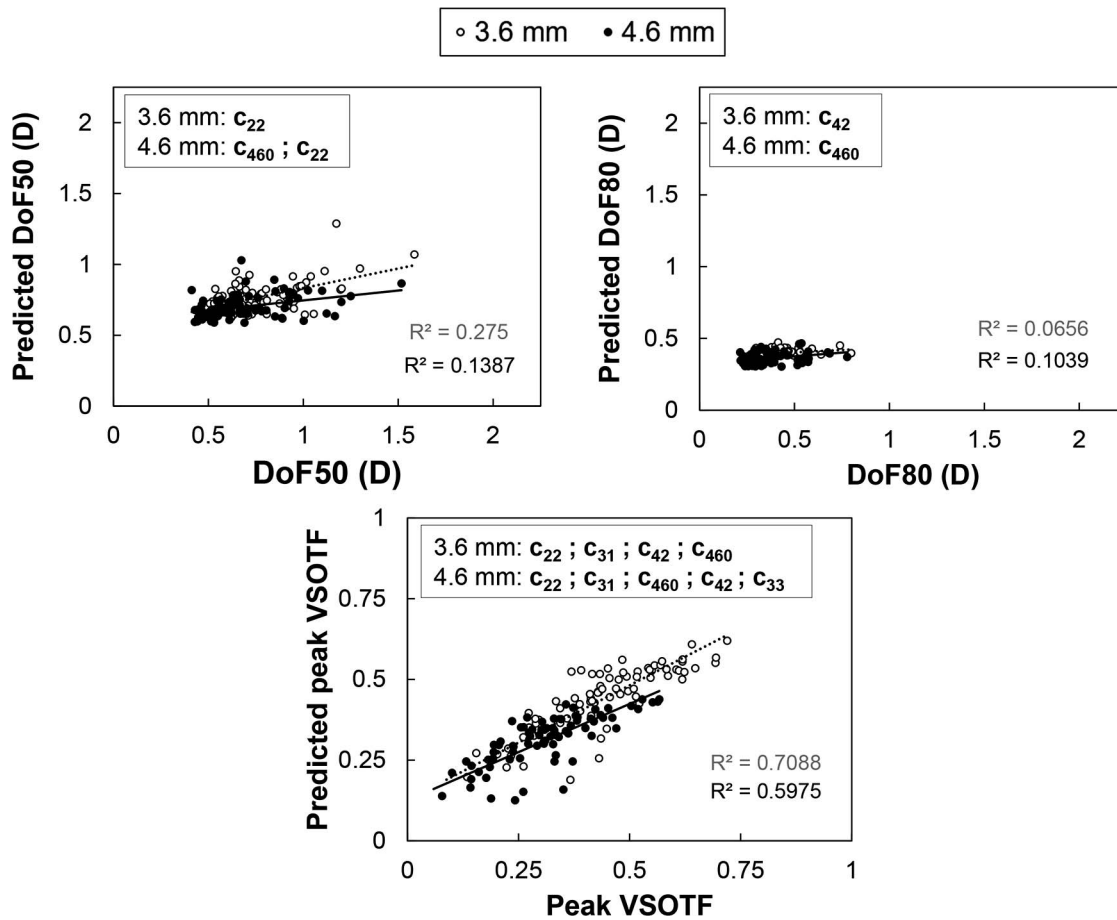
Figure 4. Correlations between the calculated depth of focus (DoF) and Peak VSOTF (considering HOAs + astigmatism), and the values predicted by the linear models for all pupils and thresholds. Solid lines represent the best linear fit to the data for a 4.6 mm pupil, whereas dotted lines correspond to the linear fit for 3.6 mm pupil. The lighter R2 corresponds to the small pupil. Notice that the axes scales can be different for each panel. Symbol c_{22} denotes second order astigmatism, c_{31} third order coma, c_{33} third order trefoil, c_{42} fourth order astigmatism, and c_{460} fourth and six order spherical aberration.
