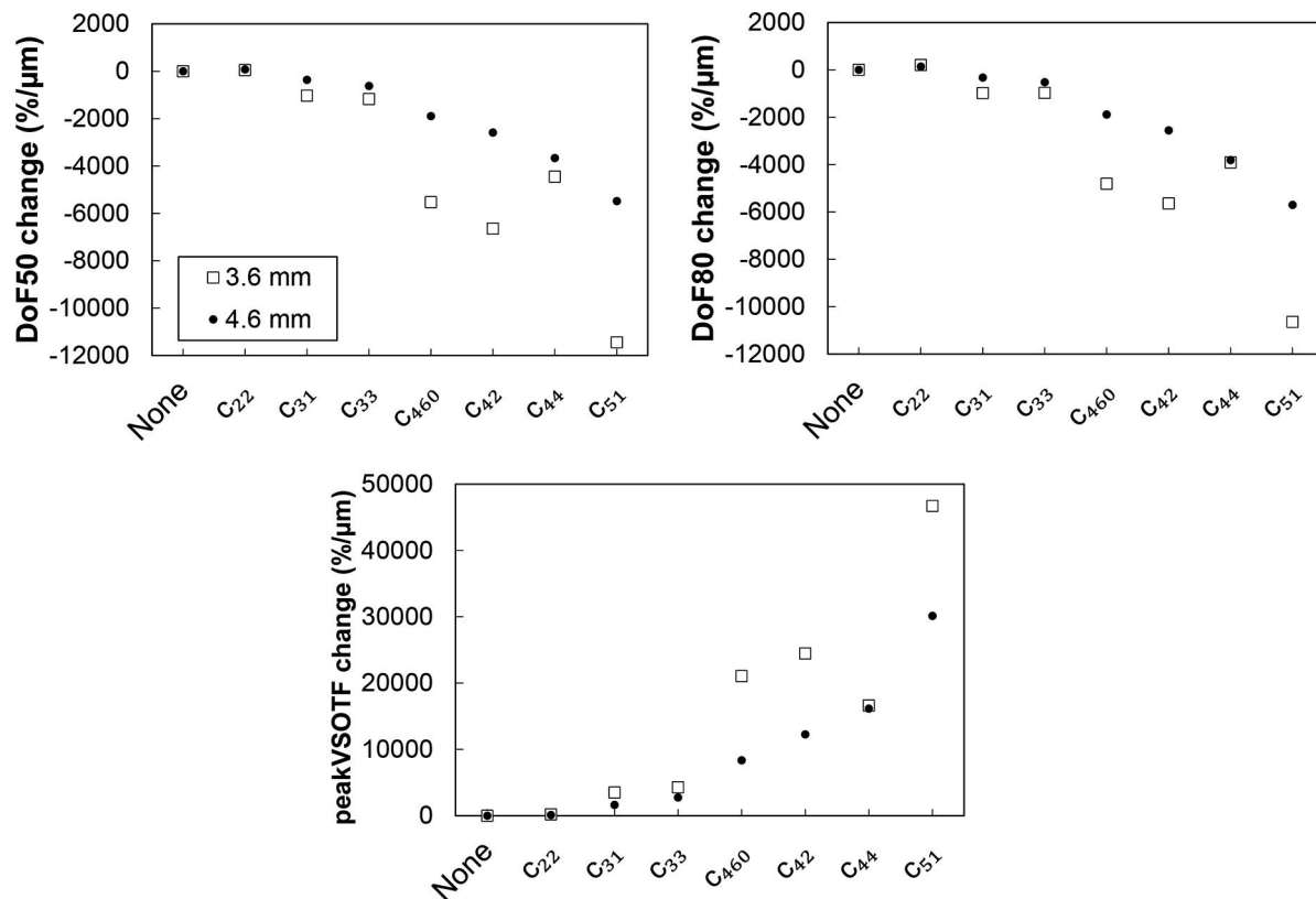
Figure 8. Top row: Change in depth of focus (DoF) for the two thresholds expressed in percentage per micron of aberrations after correcting the aberrations denoted in the X axis additively. Bottom panel: Percentage change per micrometer of aberration in the value of the Peak VSOTF after the removal of the aberrations denoted in the X axis. Error bars have been omitted for the sake of clarity. c_{22} denotes second order astigmatism, c_{31} third order coma, c_{33} third order trefoil, c_{44} fourth order tetrafoil, c_{42} fourth order astigmatism, c_{460} fourth and sixth order spherical aberration and c_{51} fifth order coma.
