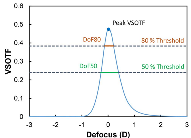
Figure 1. Estimation of the Depth of Focus (DoF) by means of the through-focus VSOTF for 50% and 80% thresholds.
