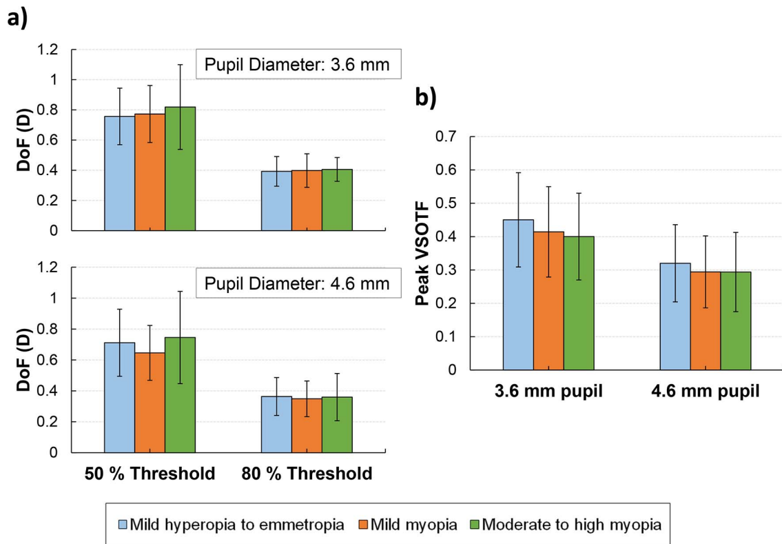
Figure 3. (a) Mean depth of focus (DoF) values for the three refractive groups calculated using a 50% and an 80% threshold. The DoF for both a 3.6 mm pupil diameter (top) and a 4.6 mm pupil diameter (bottom) is shown. (b) Peak VSOTF for the two pupil sizes and each refractive group. Error bars represent \pm one standard deviation. These values correspond to the case HOAs + astigmatism.
