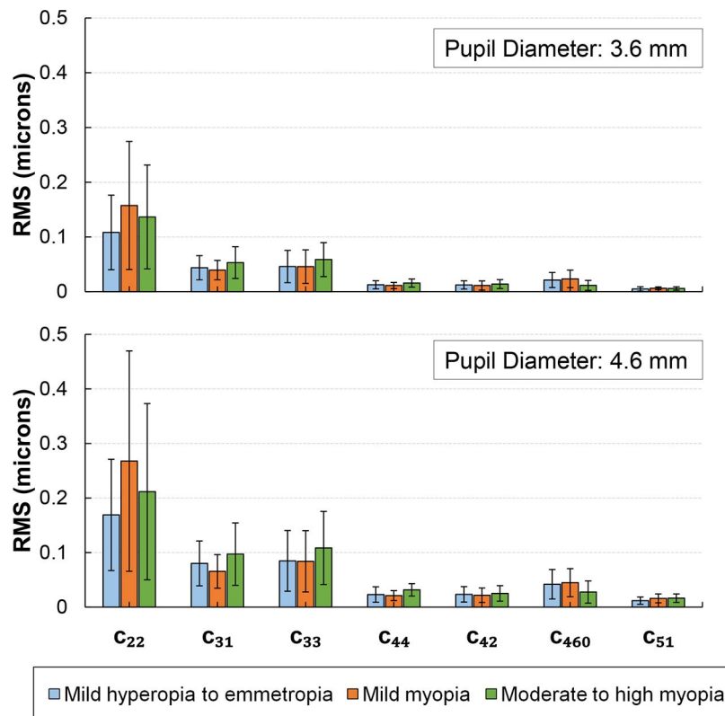
Figure 2. Mean RMS values of the grouped aberrations for each of the three refractive groups. Symbol c_{22} denotes second order astigmatism, c_{31} third order coma, c_{33} third order trefoil, c_{44} fourth order tetrafoil, c_{42} fourth order astigmatism, c_{460} fourth and sixth order spherical aberration, and c_{51} fifth order coma. Aberrations derived for both a 3.6 mm pupil diameter (top), and a 4.6 mm pupil diameter (bottom) are shown. Error bars represent \pm one standard deviation.
