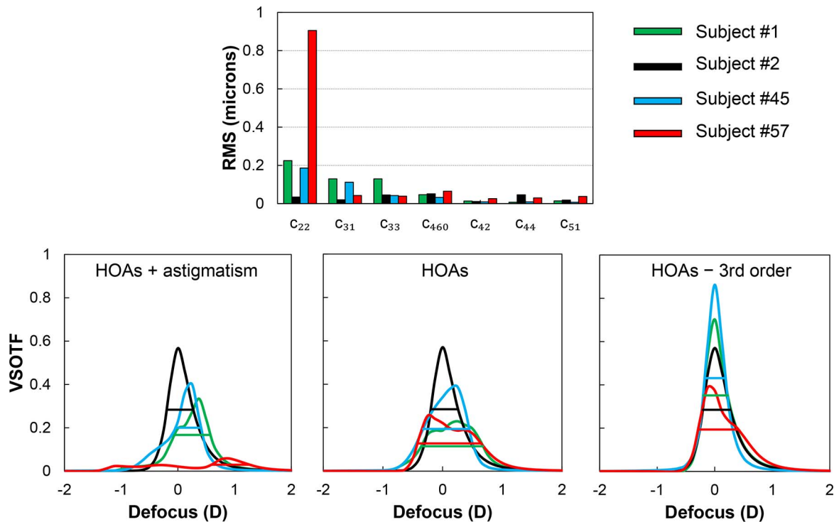
Figure 9. Top panel: RMS values in microns of each of the aberration terms considered in this study from four exemplary subjects. Bottom row: VSOTF through-focus curve and DoF50 (horizontal lines) for the same four subjects when considering different aberrations for its calculation. Symbol c_{22} denotes second order astigmatism, c_{31} third order coma, c_{33} third order trefoil, c_{44} fourth order tetrafoil, c_{42} fourth order astigmatism, c_{460} fourth and sixth order spherical aberration, and c_{51} fifth order coma.
