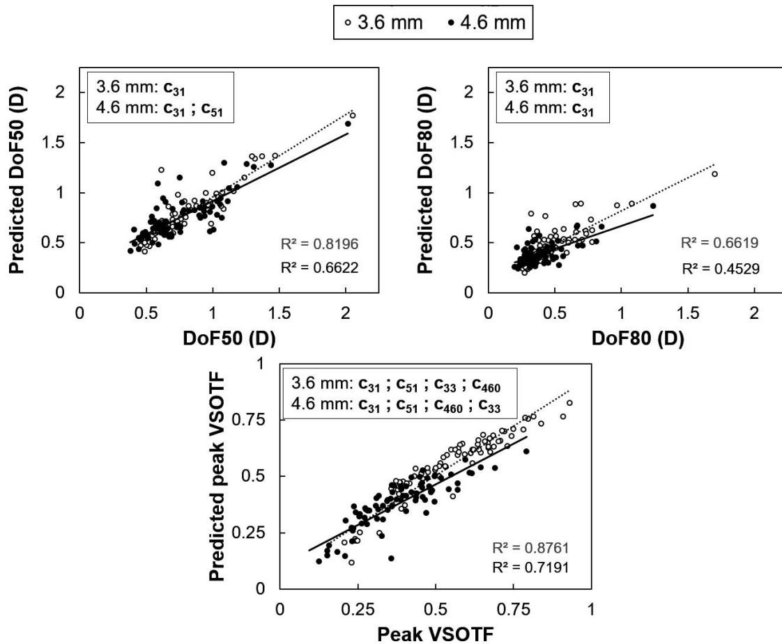
Figure 5. Correlations between the calculated depth of focus (DoF) and Peak VSOTF (considering only HOAs), and the values predicted by the linear models for all pupils and thresholds. Solid lines represent the best linear fit to the data for a 4.6 mm pupil, whereas dotted lines correspond to the linear fit for 3.6 mm pupil. The lighter R^2 value corresponds to the small pupil. Notice that the axes scales can be different. Symbol c_{31} denotes third order coma, c_{33} third order trefoil, c_{460} fourth and sixth order spherical aberration, and c_{51} fifth order coma.
