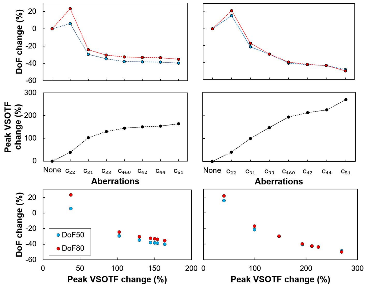
Figure 7. Top row: Change in depth of focus (DoF) expressed in percentage for all the thresholds after correcting the aberrations denoted in the x axis additively. Middle row: Percentage change in the value of the Peak VSOTF after the removal of the aberrations denoted in the x axis. Bottom row: Relationship between the change in DoF and the change in the Peak VSOTF. Columns correspond to the two different pupil diameters considered in this study: 3.6 (left) and 4.6 mm (right). Error bars have been omitted for the sake of clarity. Symbol c_{22} denotes second order astigmatism, c_{31} third order coma, c_{33} third order trefoil, c_{44} fourth order tetrafoil, c_{42} fourth order astigmatism, c_{460} fourth and sixth order spherical aberration, and c_{51} fifth order coma.
