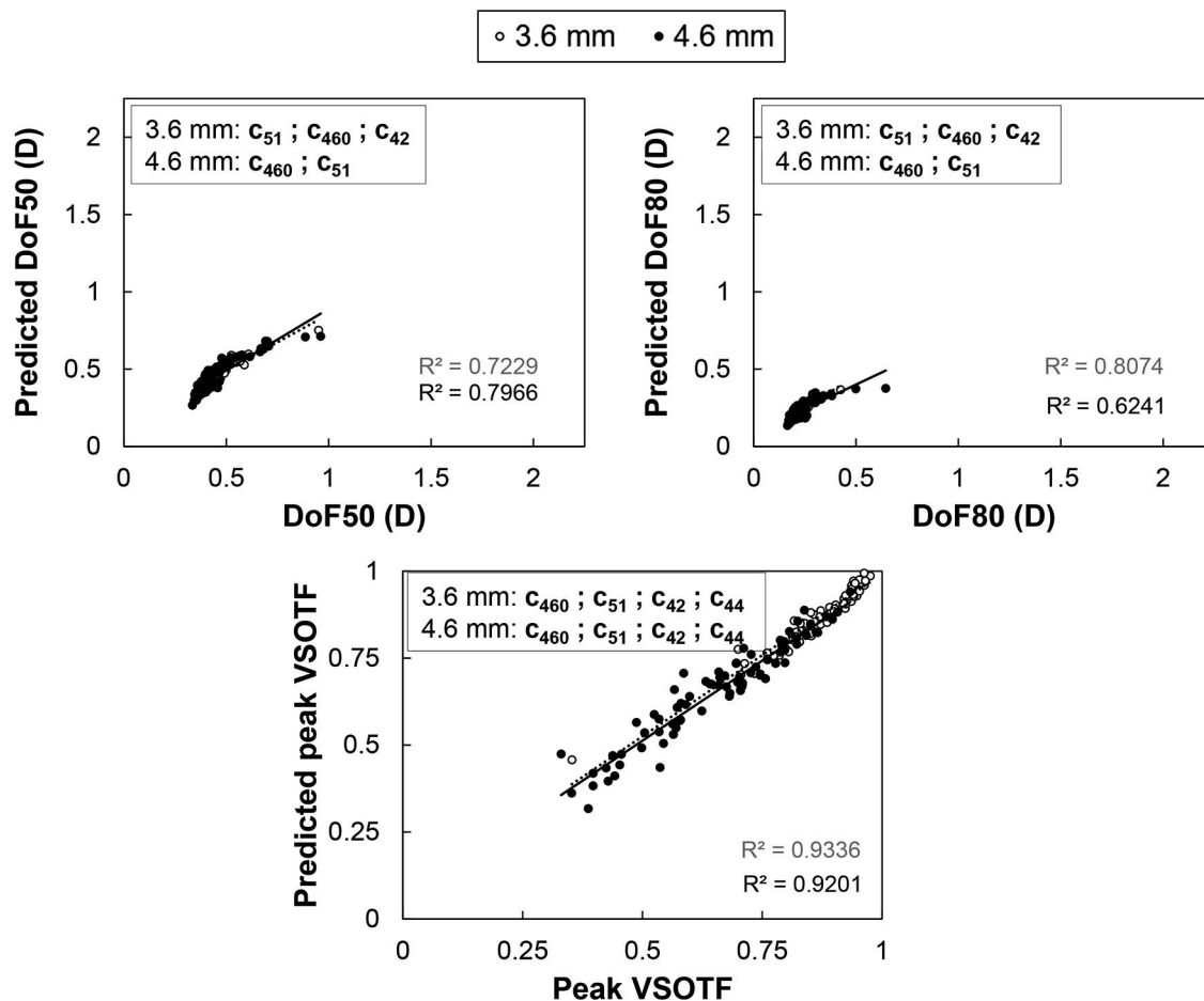
Figure 6. Correlations between the calculated depth of focus (DoF) and Peak VSOTF (HOAs – third order), and the values predicted by the linear models for all pupils and thresholds. Solid lines represent the best linear fit to the data for a 4.6 mm pupil, whereas dotted lines correspond to the linear fit for 3.6 mm pupil. The lighter R 2 value corresponds to the small pupil. Notice that the axis scales are different. Symbol c_{44} denotes fourth order tetrafoil, c_{42} fourth order astigmatism, c_{460} fourth and sixth order spherical aberration, and c_{51} fifth order coma.
