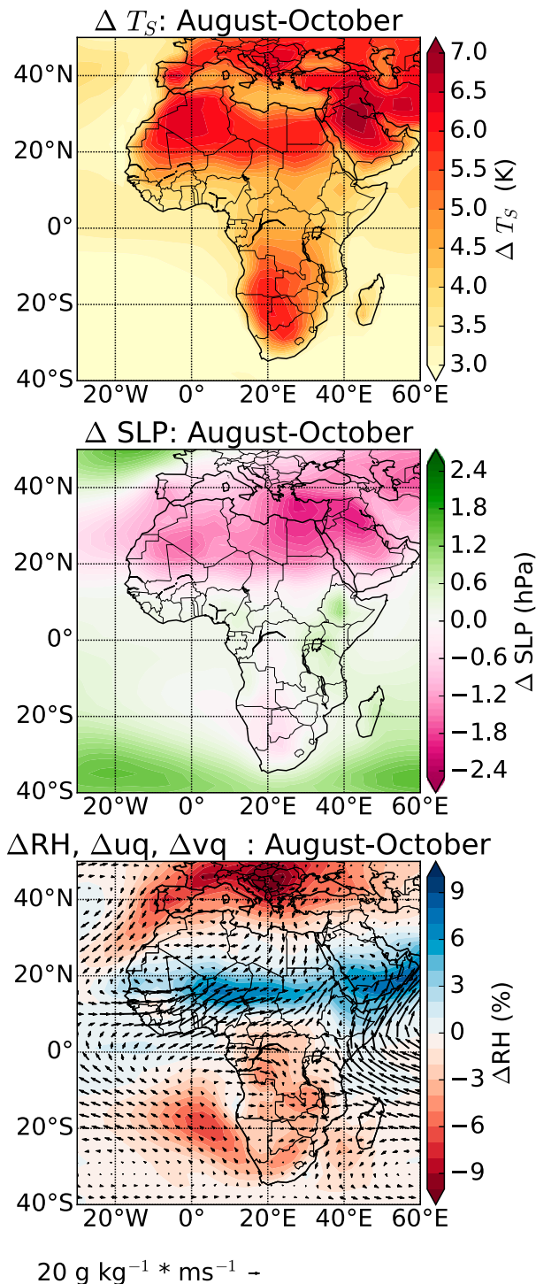
FIG. 7. Multimodel mean change in (top) surface temperature (K), (middle) sea level pressure (hPa), and (bottom) relative humidity (%) and moisture flux ( \text{g kg}^{-1} \text{m s}^{-1} ) at 925 hPa from 1980–99 (historical) to 2080–99 (RCP8.5 simulation) over August–October.
