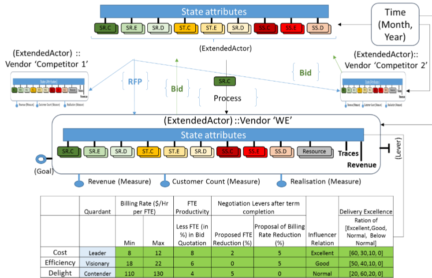
Figure 9 : Realisation of BPO scenario using EAMModel
