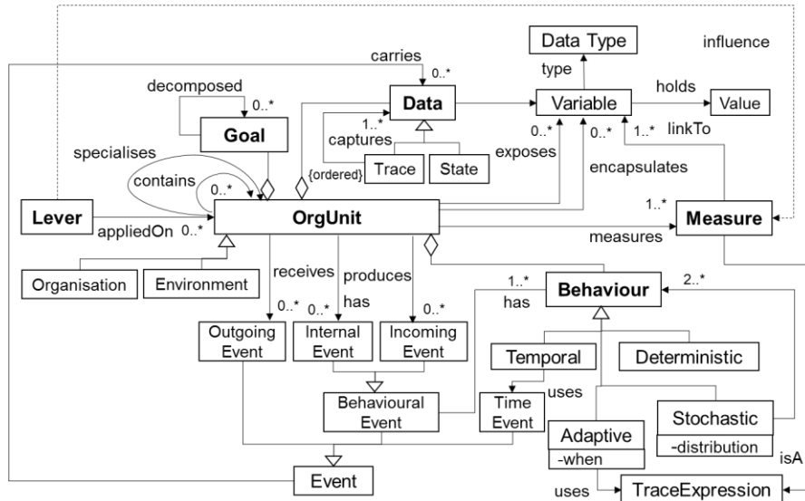
Figure 2: CMMModel – a metamodel to represent organisation
