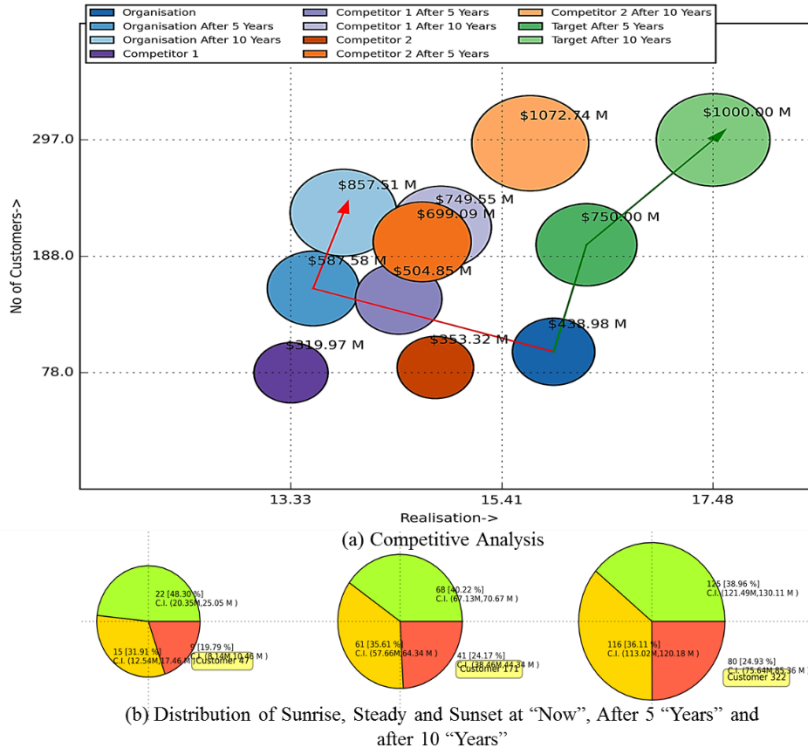
Figure 10 : Simulation Results when "WE" vendor continues as-is strategy
