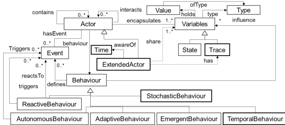
Figure 3 : ESL meta-model (ESLMMModel)
