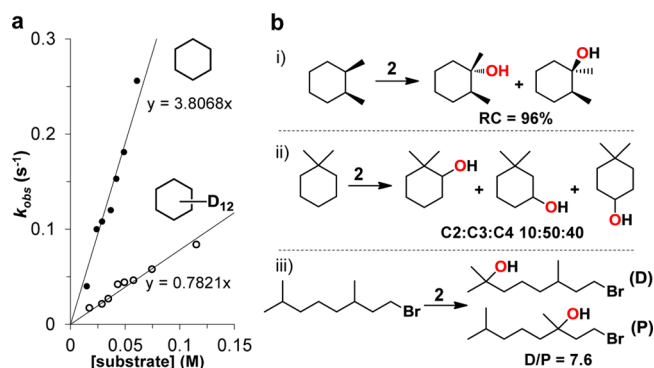
Figure 2. (a) Kinetic data for the reaction of 2 with cyclohexane at -35\text{ }^{\circ}\text{C} (cyclohexane, filled circles; cyclohexane- \text{d}_{12} , open circles). (b) Reactivity of 2 with various substrates demonstrating its selectivity.
