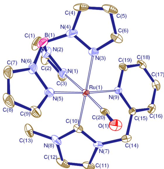
Figure 3. ORTEP diagram of the cation [TpRu( \kappa^2 -C,N-picolyl- M I)(CO)] + (picolyl- M I = 3-methyl-1-(2-picolyl)imidazol-2-ylidene) in 2a with 50% probability ellipsoids. Hydrogen atoms have been omitted for clarity. Color code: Ru, dark red; N, blue; C, brown; B, pink; O, red.
