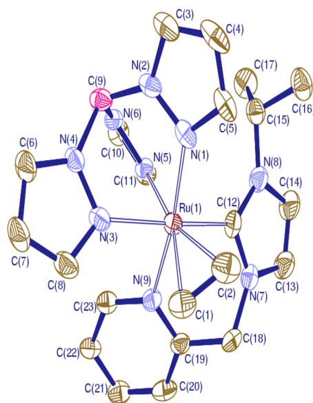
Figure 10. ORTEP diagram of the cation [\text{TpRu}(\kappa^2\text{-C}_2\text{N-picolyl-}^{\text{iPr}}\text{I})\text{-(}\eta^2\text{-CH}_2\text{=CH}_2\text{)}]^+ (picolyl- ^{\text{iPr}}\text{I} = 3 -isopropyl-1-(2-picolyl)imidazol-2-ylidene) in 5b with 50% probability ellipsoids. Hydrogen atoms have been omitted for clarity. Color code: Ru, dark red; N, blue; C, brown; B, pink.
