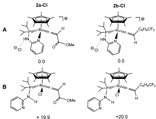
Figure 1. DFT-optimized geometries of alternative structures for compounds 2a-Cl and 2b-Cl . Relative Gibbs energies in methanol in kcal \text{mol}^{-1} .
