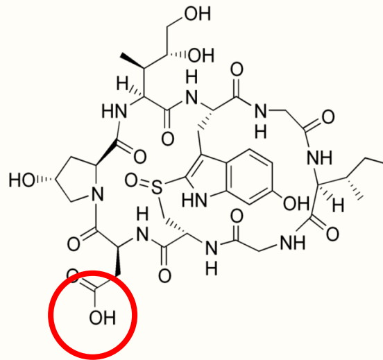
Amanitina \beta
