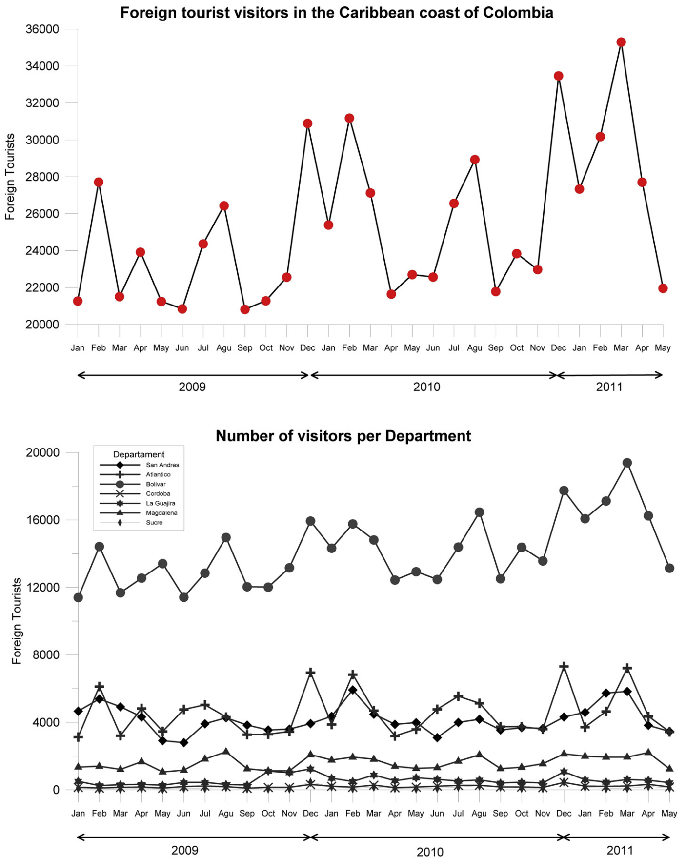
Fig. 2. Total foreign coastal tourist arrivals in the Caribbean coast Colombia (a) and data recorded at each department (b).
