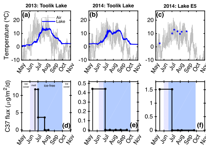
Fig. 5. Sedimentary C 37 LCA fluxes recorded in sediment traps deployed in two northern Alaskan lakes (d)–(f) plotted along with lake and air temperature data (a)–(c). Sediment fluxes were calculated for discrete sediment trap deployment periods, which lasted from 2 to 6 weeks and are delineated by the filled black circles. Shading (in (d)–(f)) represents periods of full lake ice cover (white), partial lake ice cover (light blue), and the summer ice-free period (blue).
