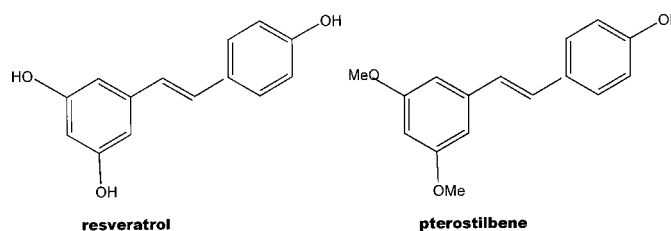
Fig. 1 Chemical structures of resveratrol and pterostilbene.
