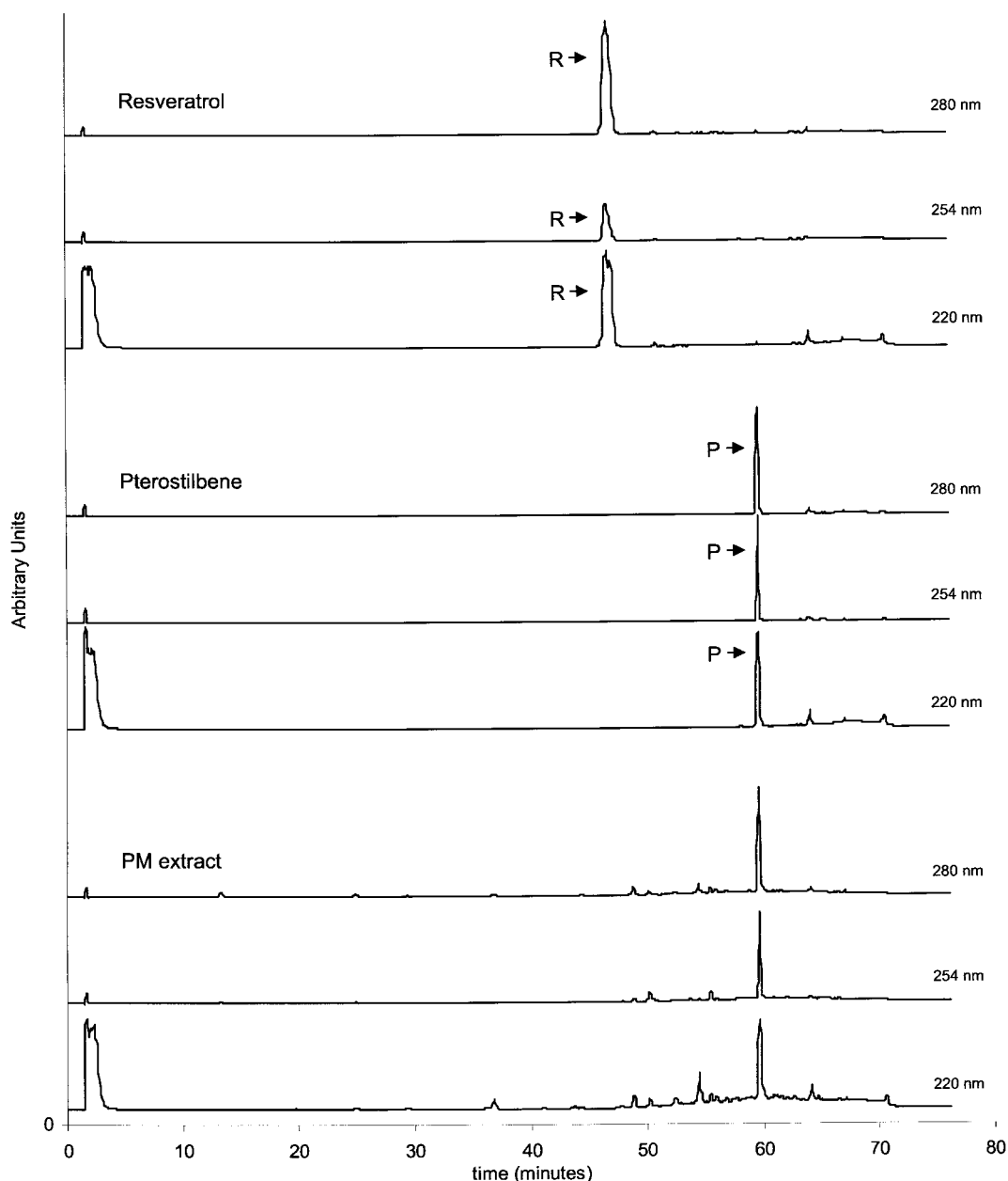
Fig. 2 HPLC chromatogram of PM extract (lower three lines), pterostilbene (middle three lines) and resveratrol (upper three lines) recorded at 220, 254 and 280 nm. With the arrows resveratrol (R) and pterostilbene (P) peaks are indicated.
