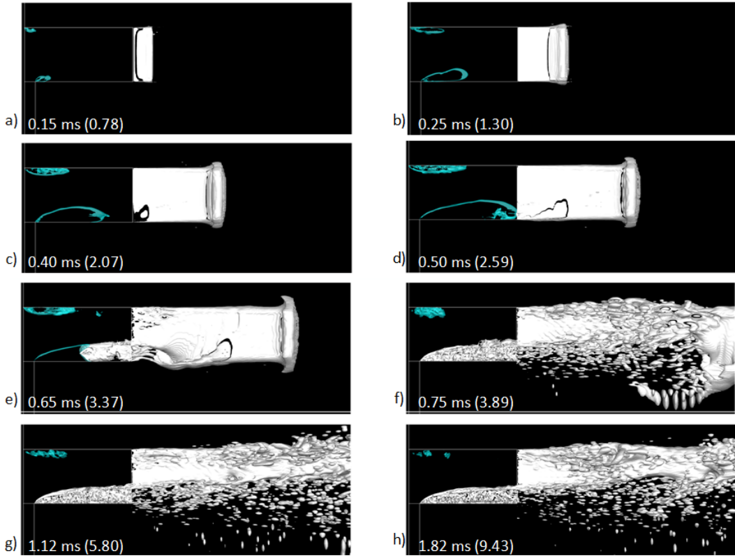
FIG. 8. Instances of the evolution of in-nozzle cavitation and liquid jet disintegration at p_{inj}=5\text{bar} . Iso-surfaces of 50% vapour (cyan) and 95% gas (white) volume fraction shown. (The non-dimensional time is given in brackets)
