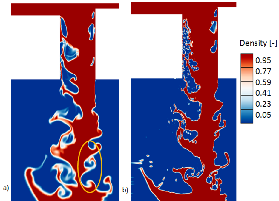
FIG. 20. Comparison between the (a)mixture approach and (b) VoF approach for modelling atomization. Contours of mixture density normalized with the water density.
