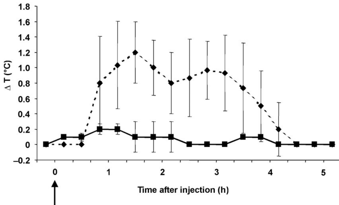
Fig. 1. Effect of IL-18 on the febrile response in rabbits. LPS (50 ng/kg) or recombinant human IL-18 (1 μg/kg) was injected intravenously into rabbits ( n = 3 per group). The body temperature (in °C measured by rectal thermometer) was measured continuously for 5 h. The arrow indicates the timepoint of the injection of LPS or IL-18.
