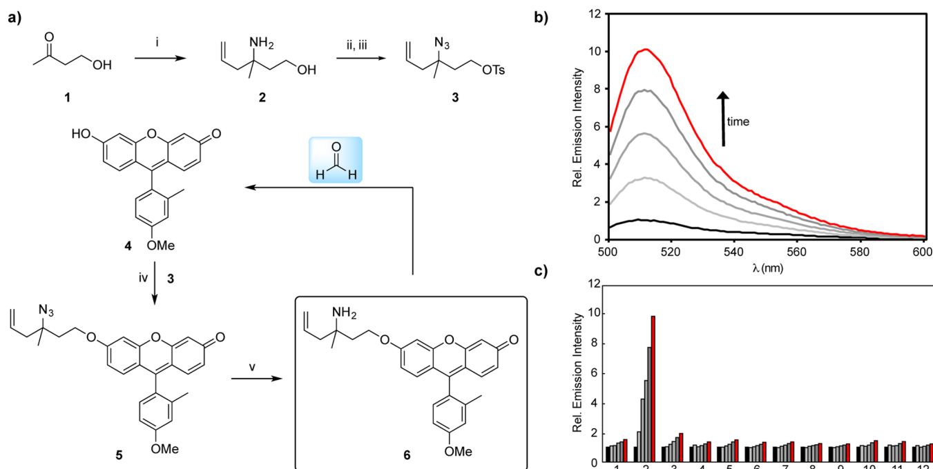
Figure 1. (a) Reagents and conditions: (i) \text{NH}_3 , MeOH, 0 °C to rt, 30 min, then allyl pinacol boronate, rt, 24 h, 69%; (ii) diazo transfer reagent, \text{CuSO}_4 \cdot 5\text{H}_2\text{O} , \text{K}_2\text{CO}_3 , MeOH, rt, 20 h; (iii) TsCl, \text{Et}_3\text{N} , DMAP, \text{CH}_2\text{Cl}_2 , rt, 16 h, 27% (2 steps); (iv) 3, \text{Cs}_2\text{CO}_3 , DMF, 40 °C, 20 h, 62%; (v) \text{SnCl}_4 , PhSH, \text{Et}_3\text{N} , MeCN, rt, 12 h, 91%. (b) Fluorescence response and selectivity of 10 μM probe 6 to 100 μM FA. Data was acquired in 20 mM PBS (pH 7.4) at 37 °C. Emission was collected between 500–600 nm ( \lambda_{\text{ex}} = 488 \text{ nm} ). Lines represent time points taken at 0 (black), 30 (light gray), 60 (gray), 90 (dark gray), and 120 min (red) after addition of 100 μM FA. (c) Fluorescence response of 10 μM probe 6 to RCS or relevant biological analyte. Data was acquired in 20 mM PBS (pH 7.4) at 37 °C. Bars represent relative emission intensity responses to 100 μM analyte after treatment for at 0 (black), 30 (light gray), 60 (gray), 90 (dark gray), and 120 min (red). Analytes were prepared as stated in the Selectivity Tests section of the SI. Legend: (1) PBS, (2) FA, (3) acetaldehyde, (4) acrolein, (5) glucose (1 mM), (6) \text{H}_2\text{O}_2 , (7) methylglyoxal, (8) dehydroascorbate (9) pyruvate, (10) glucosone, (11) oxaloacetate, (12) 4-hydroxybenzaldehyde.
