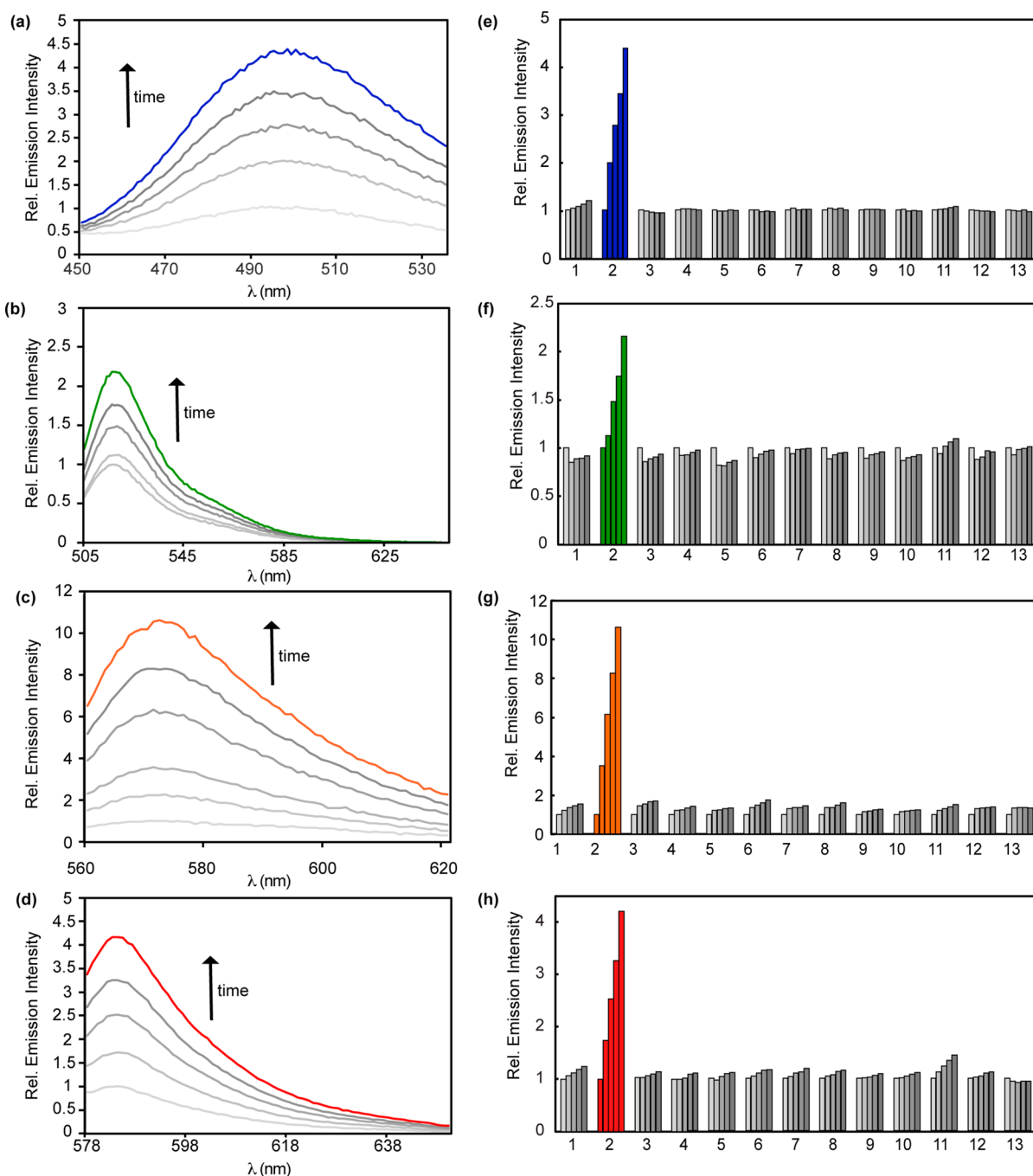
Figure 3. Fluorescence responses and selectivities of FA probes. (a–c) Fluorescence responses of 10 \mu M (a) FAP385, (b) FAP498, (c) FAP555, or (d) FAP573 to 100 \mu M FA. Data were acquired in 20 mM PBS (pH 7.4) at 37 ^{\circ} C. Emission was collected between (a) 450–535 nm ( \lambda_{\text{ex}} = 385 nm), (b) 505–645 nm ( \lambda_{\text{ex}} = 498 nm), (c) 560–625 nm ( \lambda_{\text{ex}} = 555 nm) or (d) 578–650 nm ( \lambda_{\text{ex}} = 573 nm). Lines represent time points taken at 0 (lightest gray), 30 (light gray), 60 (gray), 90 (dark gray), and 120 min (colored) after addition of 100 \mu M FA. (e–h) Fluorescence responses of 10 \mu M probe to RCS or relevant biological analyte. Bars represent emission intensity responses to 100 \mu M analyte unless otherwise stated for 0 (lightest gray), 30 (light gray), 60 (gray), 90 (dark gray), and 120 (darkest gray) min, except FA, which is shown in colored bars. Analytes were prepared as stated in the Selectivity Tests section of the SI. Legend: (1) PBS, (2) FA, (3) acetaldehyde, (4) glucose (1 mM), (5) 4-hydroxynonenal, (6) dehydroascorbate, (7) glucosone, (8) pyruvate, (9) oxaloacetate, (10) acrolein, (11) methylglyoxal, (12) H 2 O 2 , (13) glutathione (5 mM).
