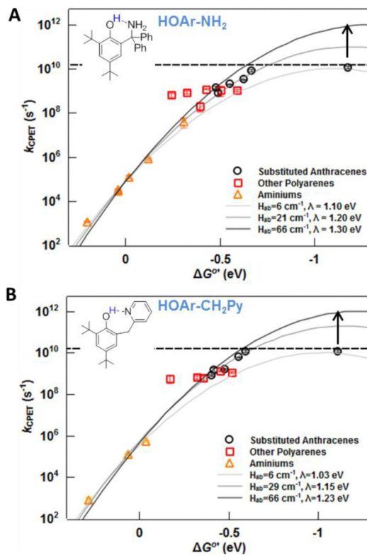
Figure 3. k_{\text{CPET}} plotted as a function of \Delta G^{0'} for (A) HOAr-NH 2 and (B) HOAr-CH 2 Py for oxidation by both excited-state polyarenes (black circles and red squares) and aminiums (orange triangles). Note the log scale on the y-axis. Various Marcus parabolas with variable \lambda have been provided with pre-exponential terms spanning 10^{10} – 10^{12} s -1 . The arrows in the plots indicate that these points, which were observed at the diffusion limit, are lower limits for k_{\text{CPET}} . The other polyarenes (red squares) are not considered in making the fits.
