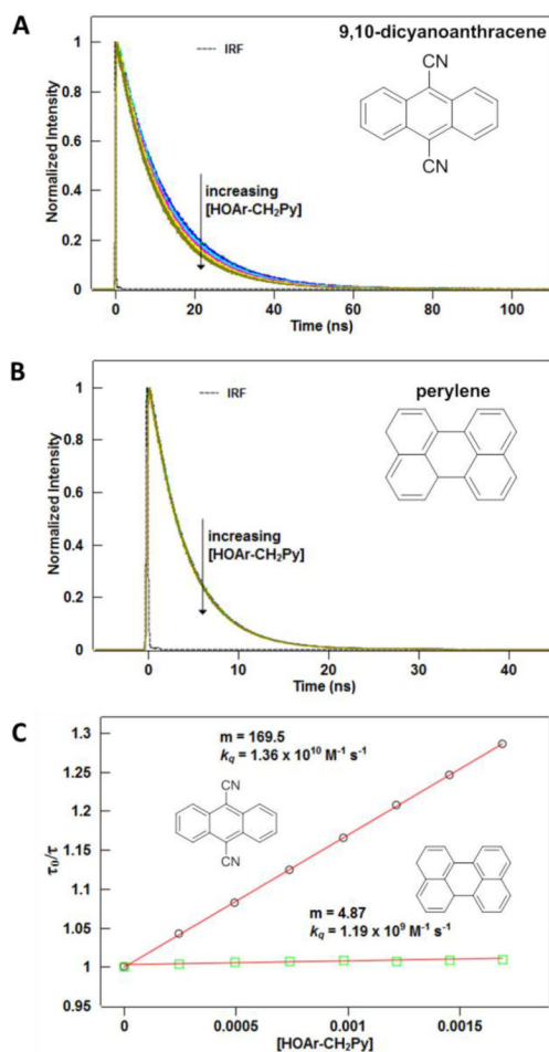
Figure 1. Examples of HOAr-CH 2 Py quenching the fluorescence of (A) 9,10-dicyanoanthracene and (B) perylene. The instrument response function (IRF), which indicates the temporal width of the excitation pulse, is shown in both cases. (C) Stern-Volmer plots for these reactions, which allow calculation of the quenching rate constant ( k_q ) from the slope (m).
