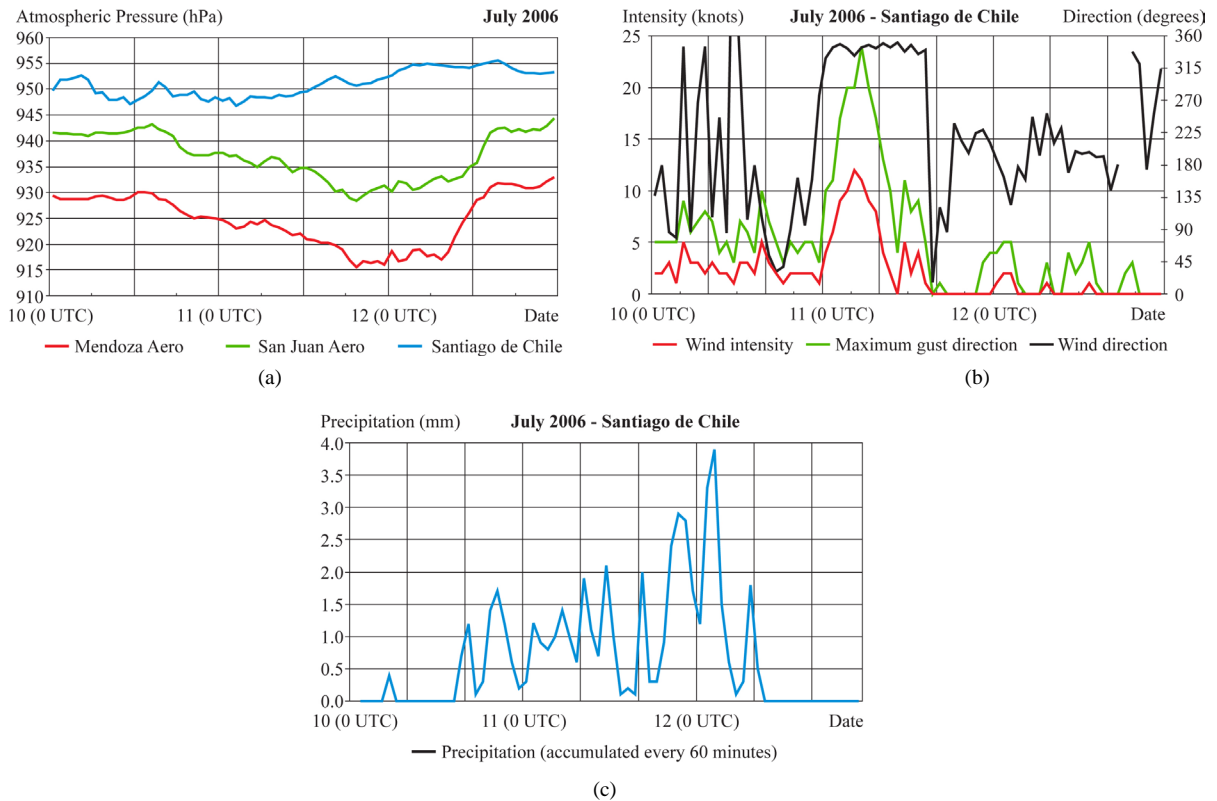
Figure 14. (a) Atmospheric pressure evolution in Santiago de Chile, Mendoza Aero and San Juan Aero; (b) Wind velocity, maximum gusts and wind direction in Santiago de Chile; (c) Accumulated precipitation in Santiago de Chile. All before, during and after zonda event of July 11 th , 2006.
