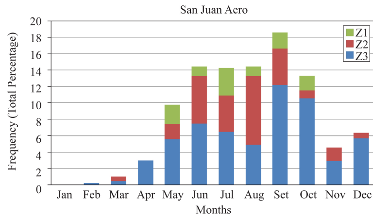
Figure 31. Monthly frequency (by intensity) of zonda in San Juan Aero.
