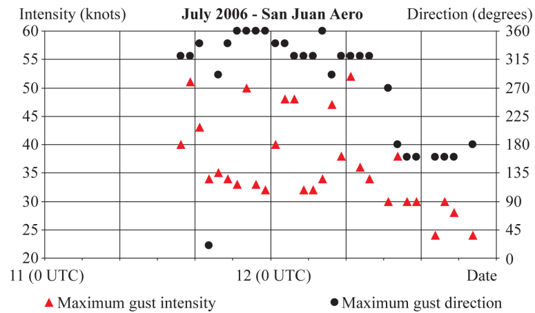
Figure 12. Maximum gust and gust direction during zonda event of July 11 th , 2006, in San Juan Aero.
