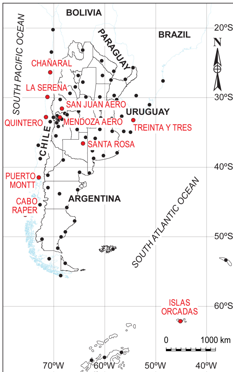
Figure 36. South America map showing the 81 meteorological stations used for the probabilistic prediction and those selected by SDA.
