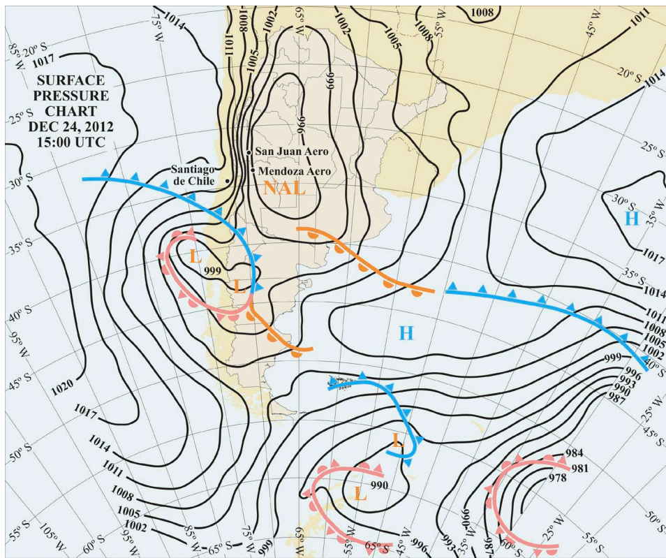
Figure 15. Surface synoptic situation at 15 UTC on December 24 th , 2012.
