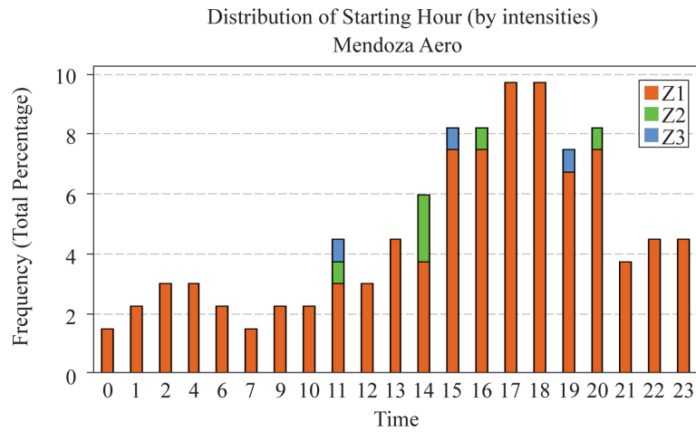
Figure 28. Time of onset of zonda events (by intensities) in Mendoza Aero.
