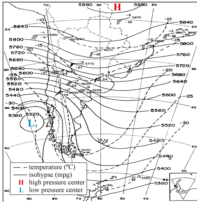
Figure 7. 500 hPa level chart at 12 UTC on August 23 rd , 1983.
