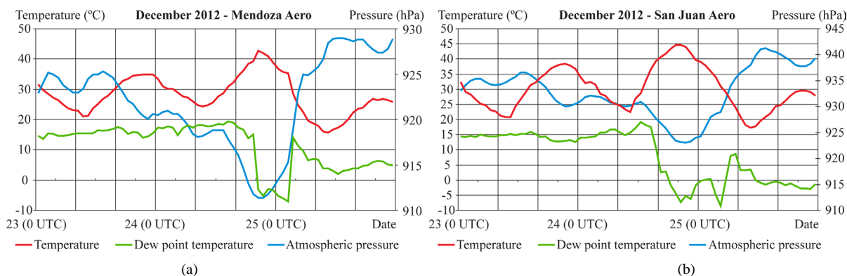
Figure 20. Atmospheric pressure, temperature and dew point evolution before, during and after leeside zonda event of December 24 th , 2012: (a) in Mendoza Aero; (b) in San Juan Aero.
