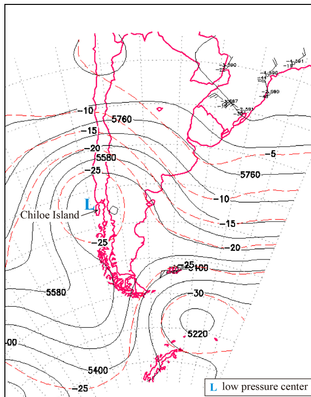
Figure 18. 500 hPa level chart at 0 UTC on December 25 th , 2012.
