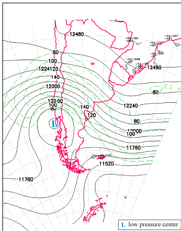
Figure 19. 200 hPa level chart at 0 UTC on December 25 th , 2012.
