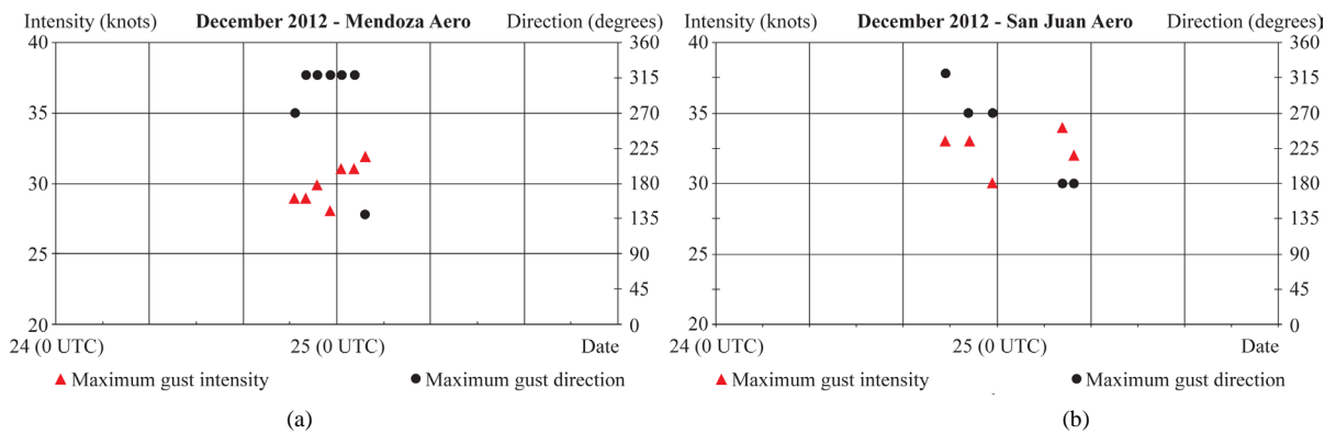
Figure 22. Maximum gust and gust direction during zonda event of December 24 th , 2012: (a) in Mendoza Aero; (b) in San Juan Aero.
