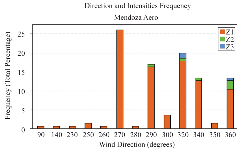
Figure 30. Frequency of direction of zonda events in Mendoza Aero.
