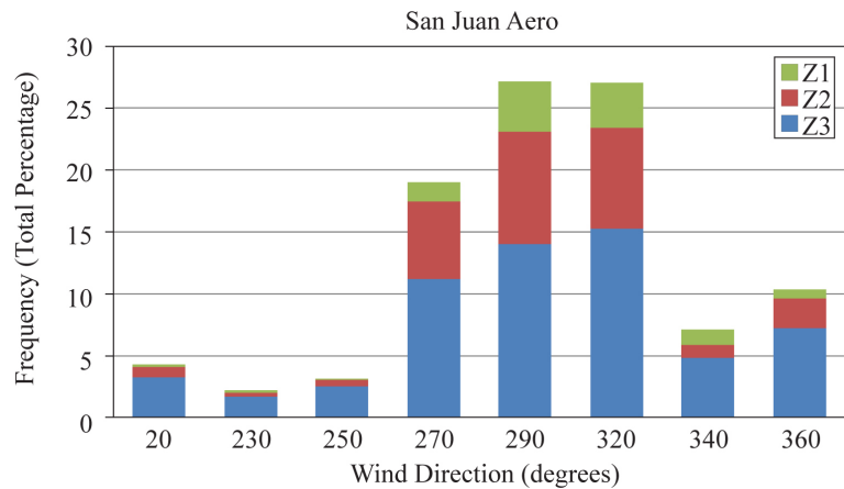
Figure 34. Frequency of direction of zonda events in Mendoza Aero.
