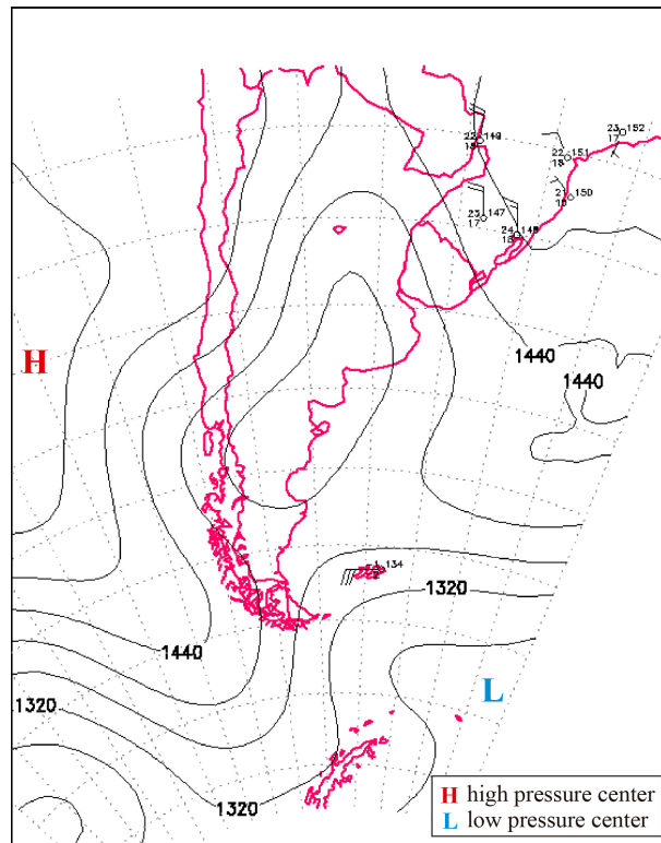
Figure 17. 850 hPa level chart at 0 UTC on December 25 th , 2012.
