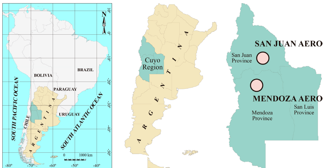
Figure 1. Location of Argentina and Cuyo region in South America.
