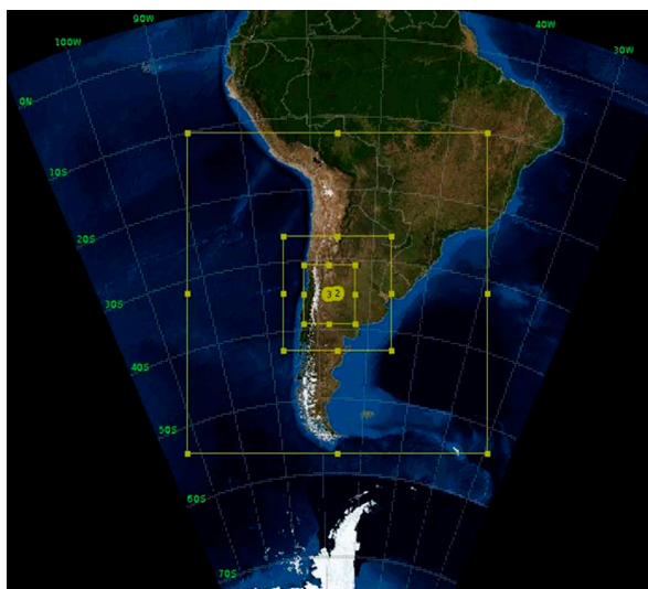
Figure 3. WRF model setting specification.
