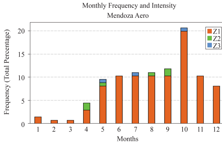
Figure 27. Monthly frequency (by intensity) of zonda in Mendoza Aero.
