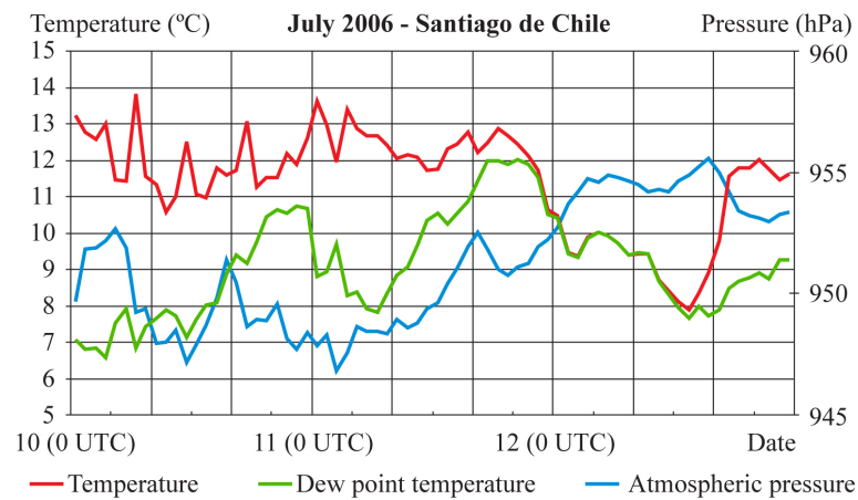
Figure 13. Atmospheric pressure, temperature and dew point evolution before, during and after leeside zonda event of July 11 th , 2006, in Santiago de Chile.
