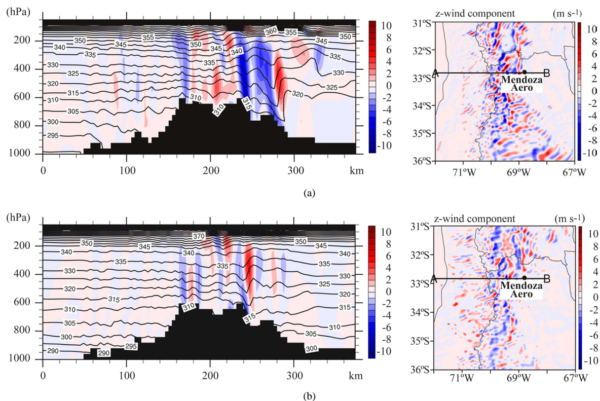
Figure 26. Horizontal and vertical analysis of gravity waves and potential temperature at Mendoza Aero latitude: (a) on December 24 th , 2012; (b) on December 17 th , 2012.
