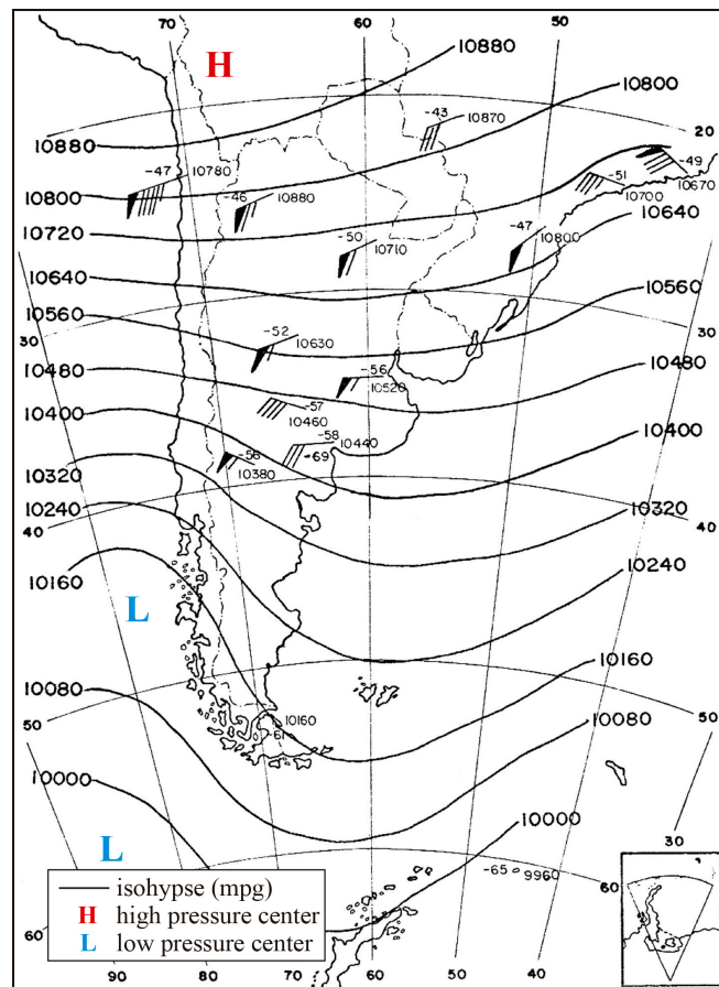
Figure 8. 200 hPa level chart at 12 UTC on August 23 rd , 1983.
