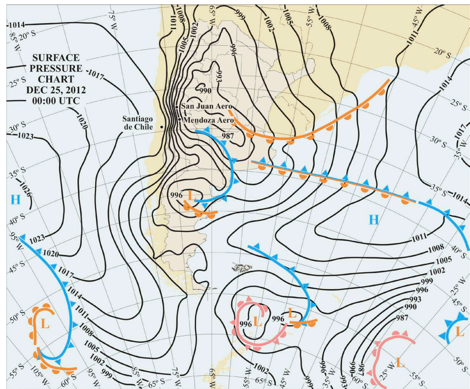
Figure 16. Surface synoptic situation at 0 UTC on December 25 th , 2012.
