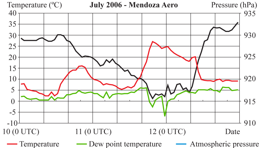
Figure 9. Atmospheric pressure, temperature and dew point evolution before, during and after zonda event of July 11 th , 2006, in Mendoza Aero.
