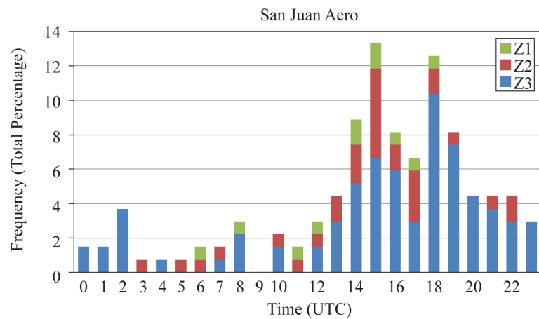
Figure 32. Time of onset of zonda events (by intensities) in San Juan Aero.
