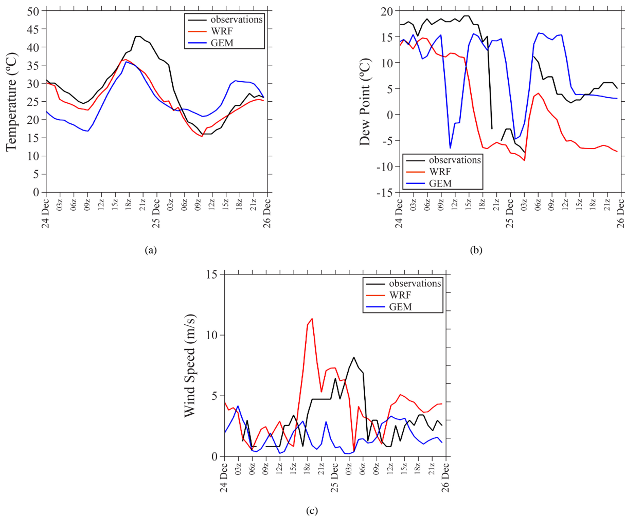
Figure 38. (a) Surface temperature; (b) Dew point; (c) Wind speed. All observed and forecasted by WRF and GEM models for the summer severe event of December 24 th , 2012, for Mendoza Aero.
