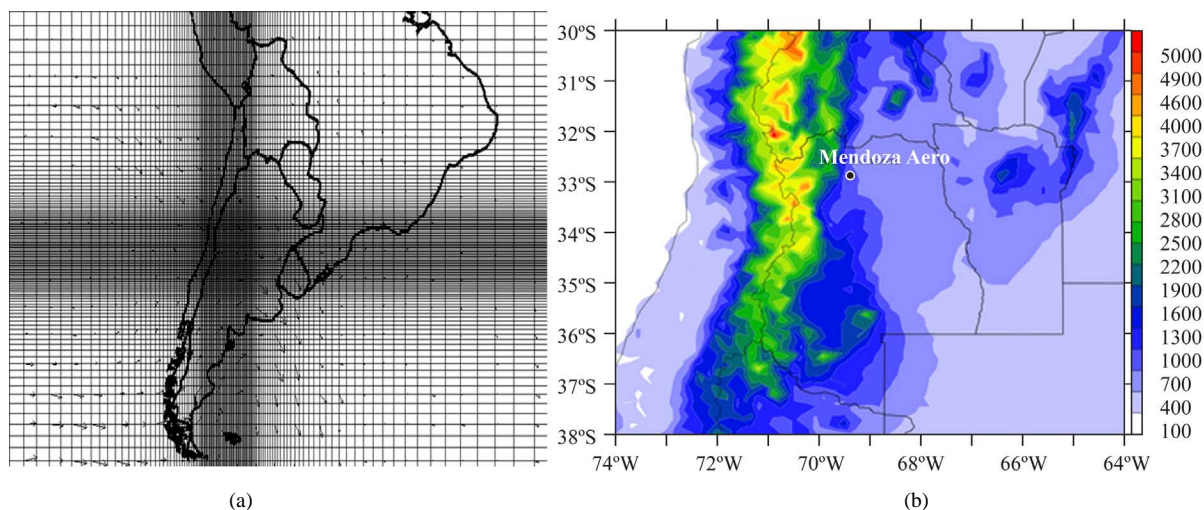
Figure 2. (a) Stretched grid section (centered at Mendoza province) of the global domain; and (b) the topography used by GEM model.
