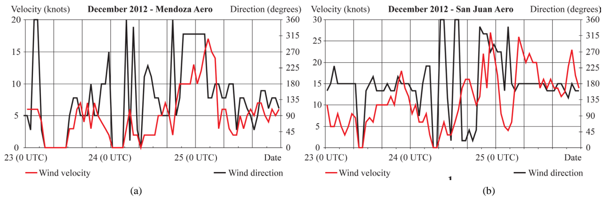
Figure 21. Velocity and wind direction evolution before, during and after zonda event of December 24 th , 2012: (a) in Mendoza Aero; (b) in San Juan Aero.
