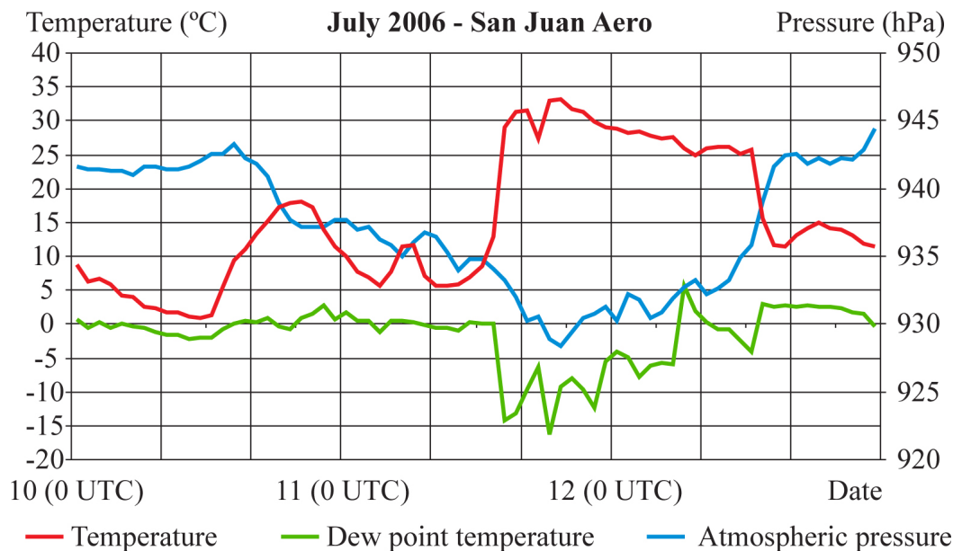
Figure 10. Atmospheric pressure, temperature and dew point evolution before, during and after zonda event of July 11 th , 2006, in San Juan Aero.
