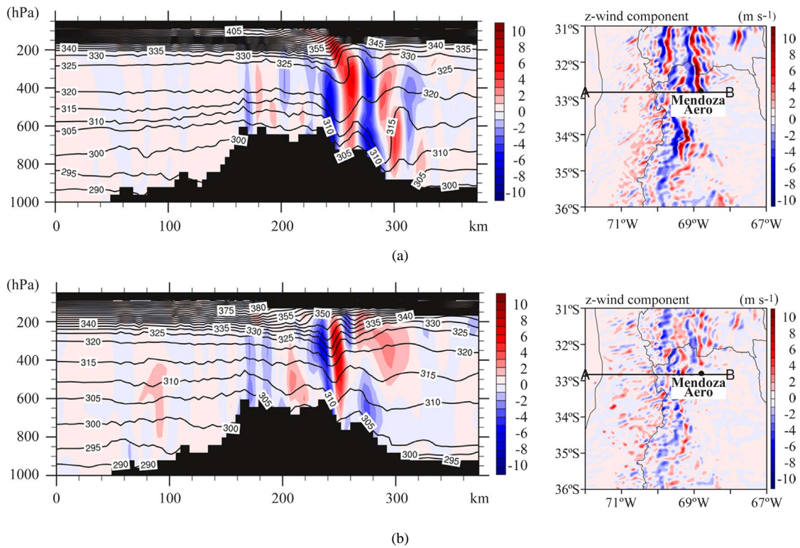
Figure 25. Horizontal and vertical analysis of gravity waves and potential temperature at Mendoza Aero latitude: (a) on July 11 th , 2006; (b) on June 12 th , 2012.
