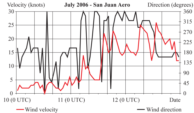
Figure 11. Evolution of wind velocity and direction before, during and after zonda event of July 11 th , 2006, in San Juan Aero.
