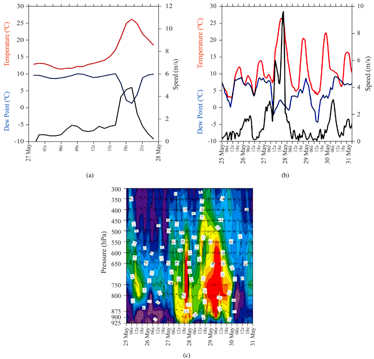
Figure 37. (a) Wind speed, temperature and dew point before, during and after de FNZ1 zonda event of May 27 th , 2012, on Mendoza Aero; (b) Forecasted surface parameters using GEM model for the zonda event of May 27 th , 2012, on Mendoza Aero.; (c) Forecasted dew point depression on the vertical axis using GEM model.
