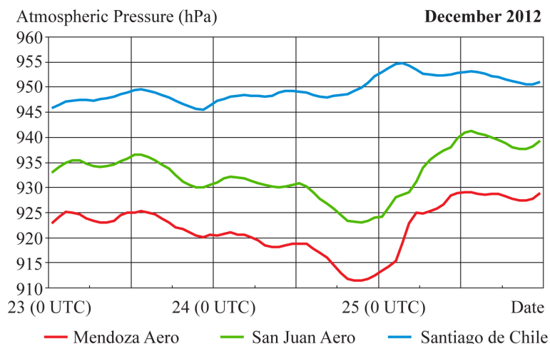
Figure 24. Atmospheric pressure evolution in Santiago de Chile, Mendoza Aero and San Juan Aero before, during and after leeside zonda event of December 24 th , 2012.
