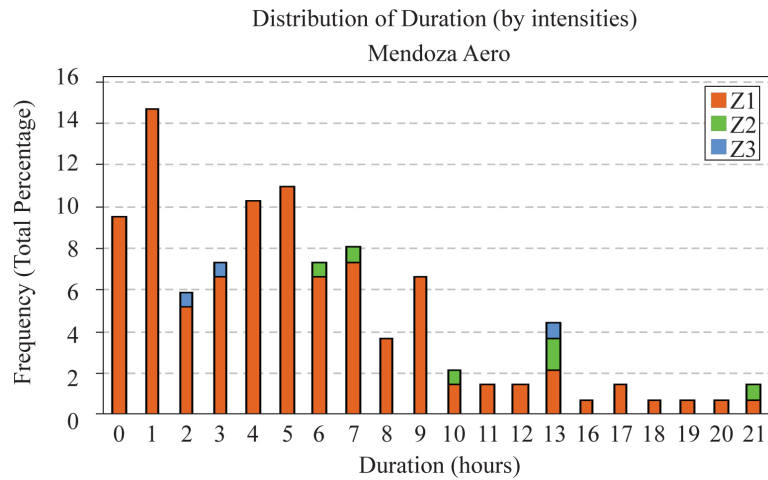
Figure 29. Frequency of duration (in hours) of zonda events in Mendoza Aero.
