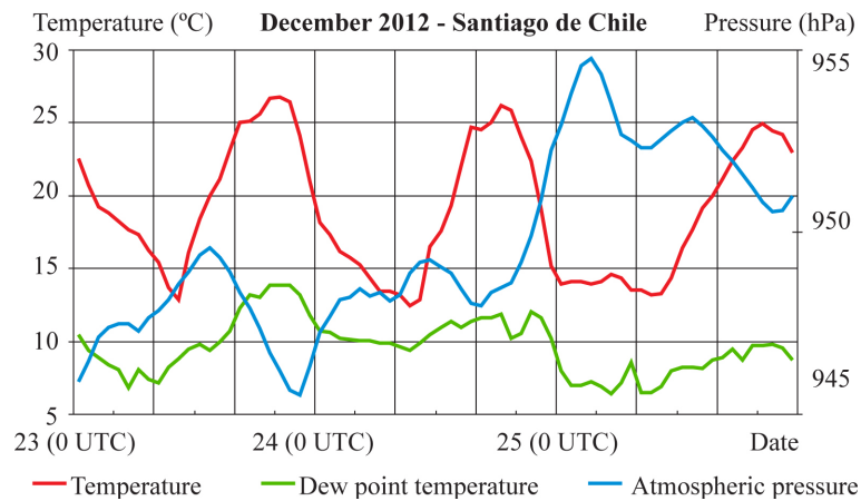
Figure 23. Atmospheric pressure, temperature and dew point evolution before, during and after leeside zonda event of December 24 th , 2012, in Santiago de Chile.
