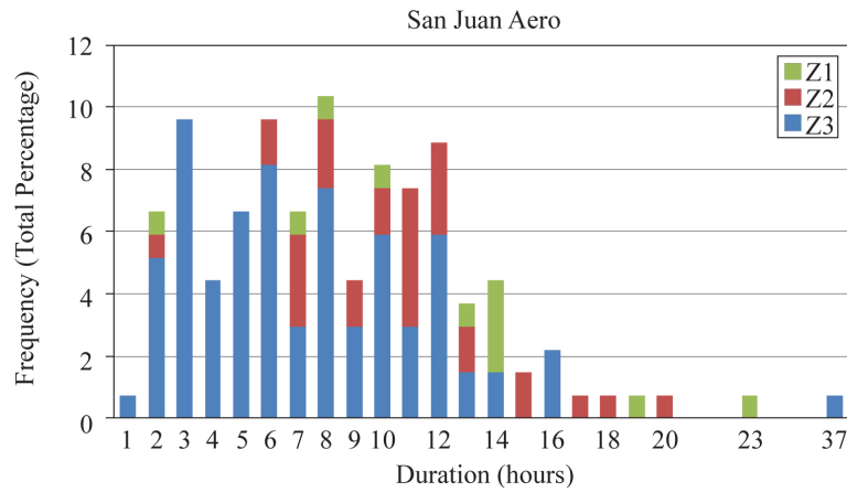
Figure 33. Frequency of duration (in hours) of zonda events in San Juan Aero.
