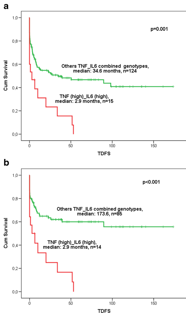
Fig. 2 Transfusion dependence-free survival (TDFS) and combined genotypes. Kaplan-Meier curves indicating the median TDFS with respect to TNF_IL6 combined genotypes for (a) the overall MDS population and (b) patients with <5% bone marrow blasts
