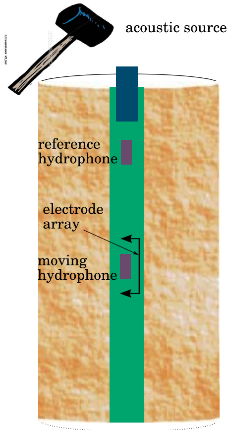
Figure 25. Scheme of the principle of electrokinetic logging to measure the permeability (modified from Singer et al., 2005, in Jouniaux, 2011). The acoustic source induces a Stoneley wave propagation (detected by the hydrophones) leading to an electric field (measured by the electrodes). The experiment is repeated by moving the tool downward.
