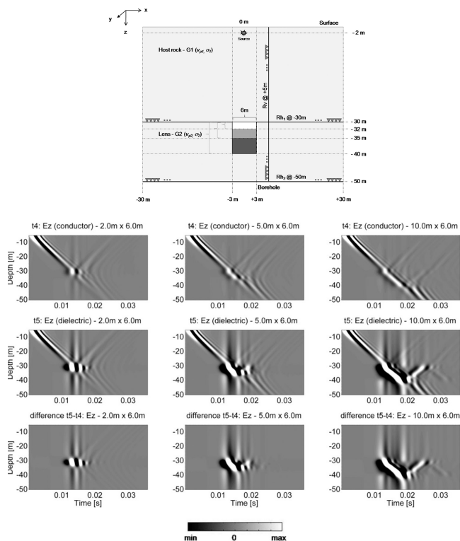
Figure 13. Model and electrograms for the following confined unit geometries: the left column is for 2\text{ m} \times 6\text{ m} the middle column is for 5\text{ m} \times 6\text{ m} and the right column is for 10\text{ m} \times 6\text{ m} . The top row shows the z component of the electric field for a the material with electrical conductivity of 0.05\text{ S m}^{-1} , the middle row shows the z component of the electric field for a material with electrical conductivity of 10^{-5}\text{ S m}^{-1} . The bottom row shows the calculated differences in the amplitudes for both previous models. Notice that all amplitudes are scaled identically and that the electric conductivity is the only medium parameter with contrasts among different units (from Kröger et al., 2014).
