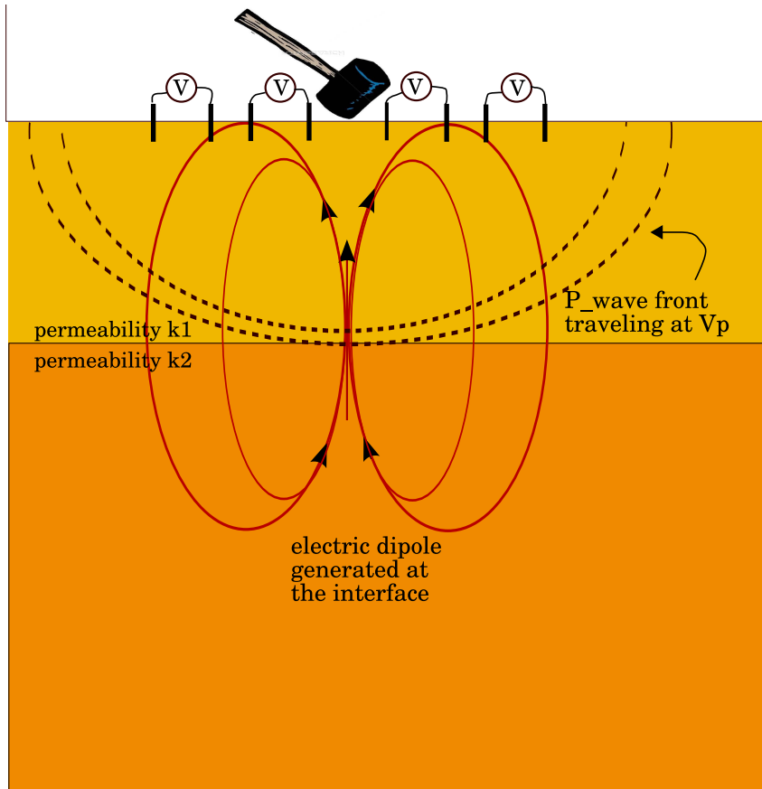
Figure 3. The seismic waves propagate up to the interface where an electric dipole is generated because of the contrast in permeability. This electromagnetic wave can be detected at the surface by measuring the difference of the electrical potential V between electrodes. Picking the time arrival allows to know the depth of the interface (from Jouniaux and Ishido, 2012).
