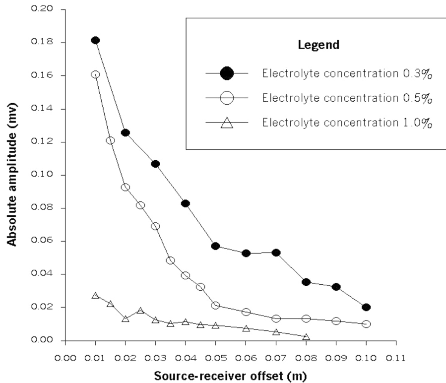
Figure 17. The amplitude of the first kind of seimo-electric conversion as a function of the source-receiver offset. The electrolyte concentration is NaCl concentration (from Chen and Mu, 2005).
