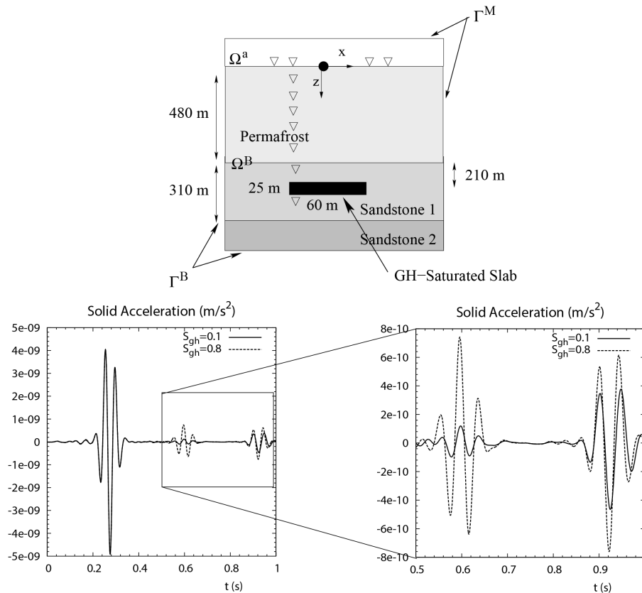
Figure 12. SHTe-mode solid acceleration traces for different gas hydrates reservoir saturations, for the shown model. The first wave train corresponds to the conversion generated at the permafrost base, the second one to the conversions at the slab – top and bottom IR's are indistinguishable one from each other – and finally, the wavetrain arriving at about 0.9 s is the reflection on the slab of the seismic waves originated on the permafrost/sandstone interface (from Zyserman et al., 2012).
