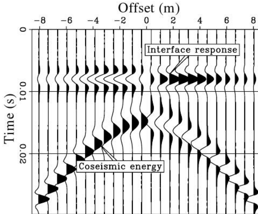
Figure 4. Model of the seismolectric response to a hammer strike on the surface at position zero (from Haines, 2004). The seismolectric signal is shown as measured at the surface along a line centered on the seismic source. The interfacial signal is related to a contrast between properties of the media, such as the permeability.
