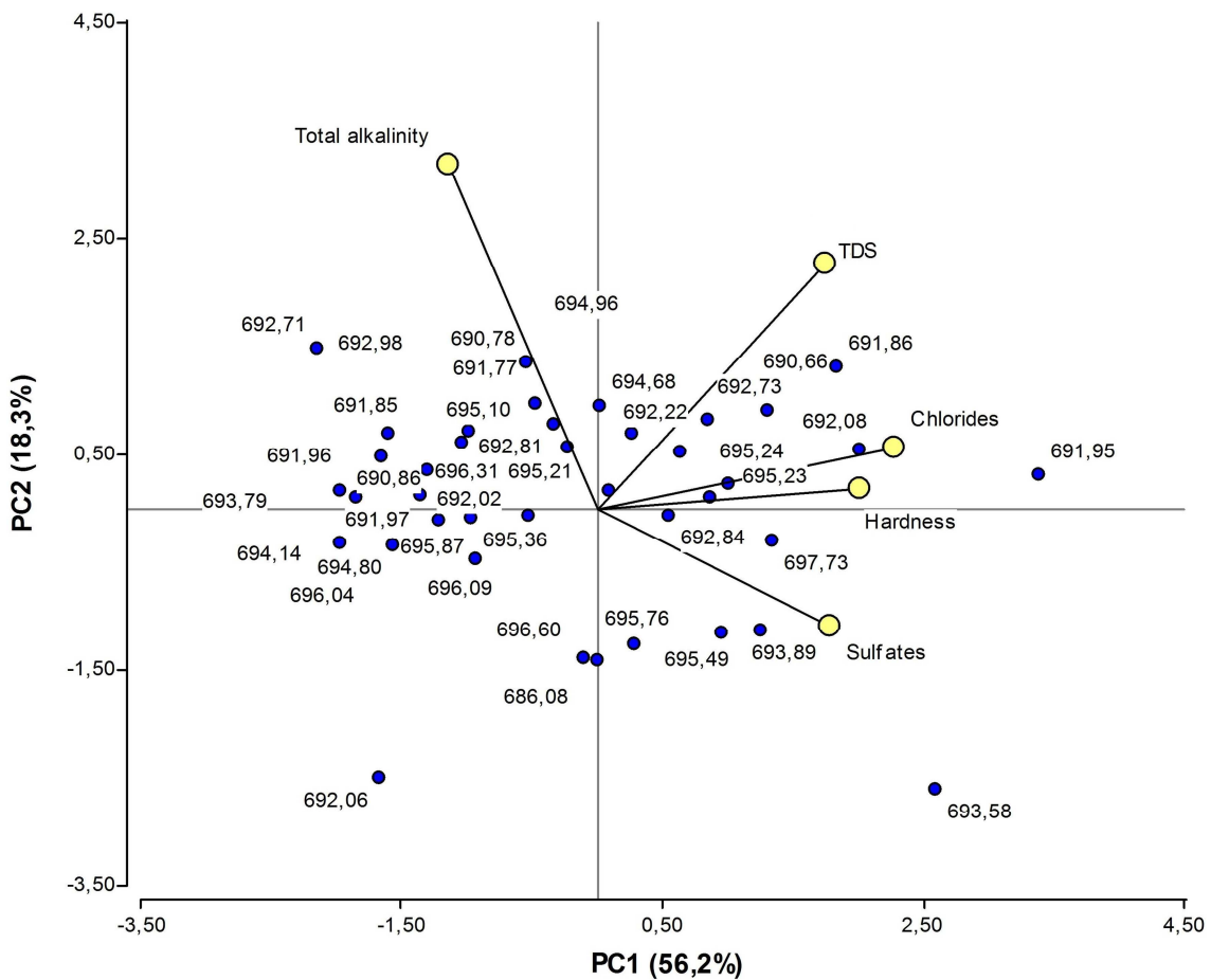
Figure 3. Multivariate analysis of characterization parameters and GPS vector coordinates.
