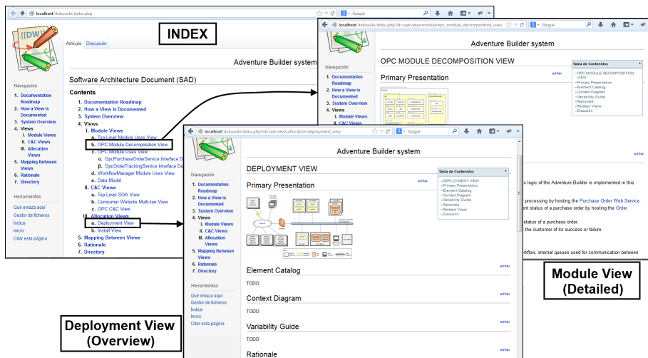
Fig. 1 Example of a Wiki-based SAD for a system called AdventureBuilder
