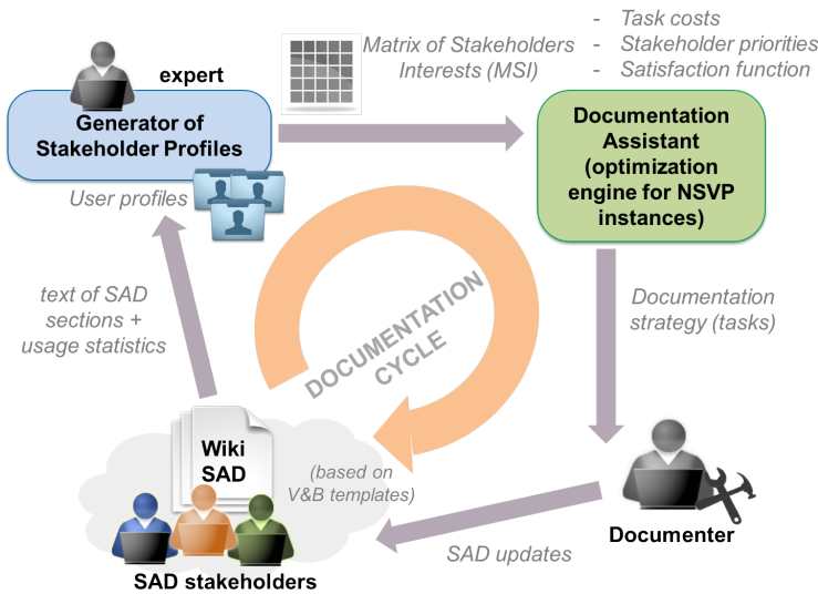
Fig. 3 ProSAD: an architecture documentation driven by stakeholders' concerns.
