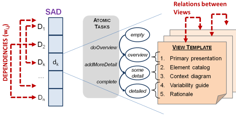
Fig. 4 Documentation tasks for a SAD section, based on the V&B view templates
