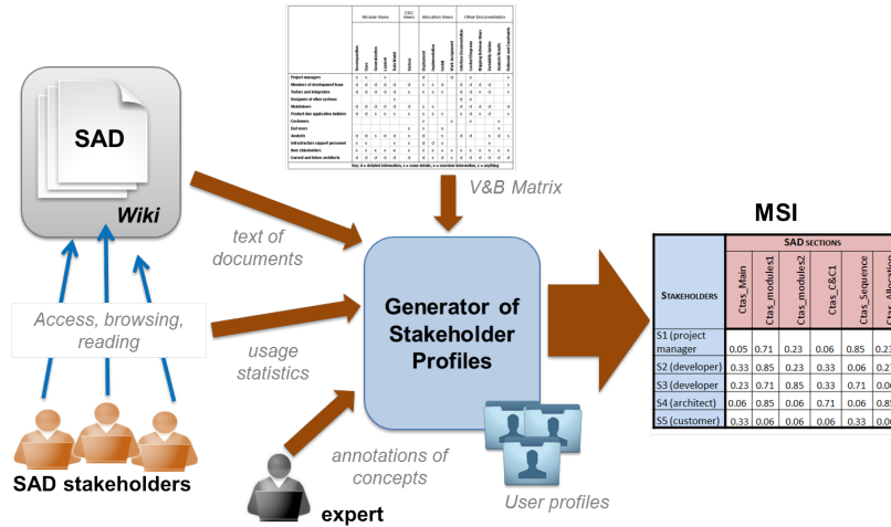
Fig. 11 Pipeline for constructing stakeholder profiles and updating the MSI
