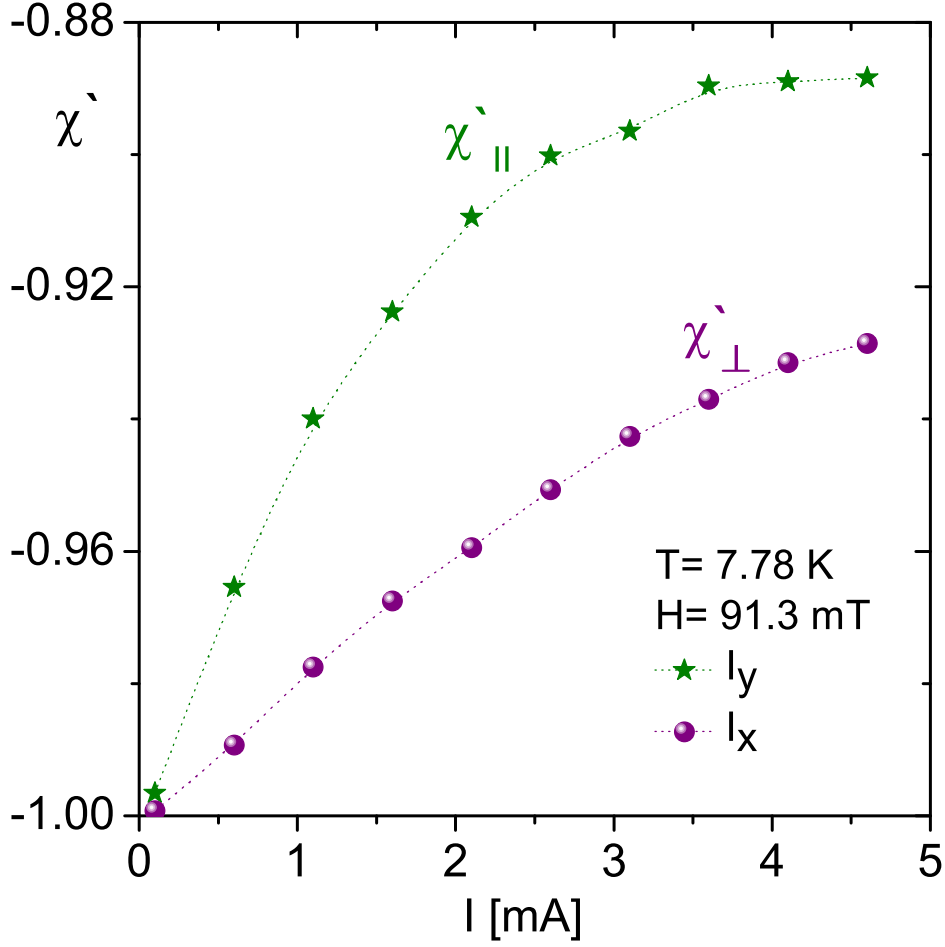
Fig. 3. Real part of the susceptibility as a function of the bias current for both current orientations at a fixed value of magnetic field. The temperature of these measurements was at the minimum of the susceptibility at zero current, T_p , indicated with an arrow in Figure 2.
