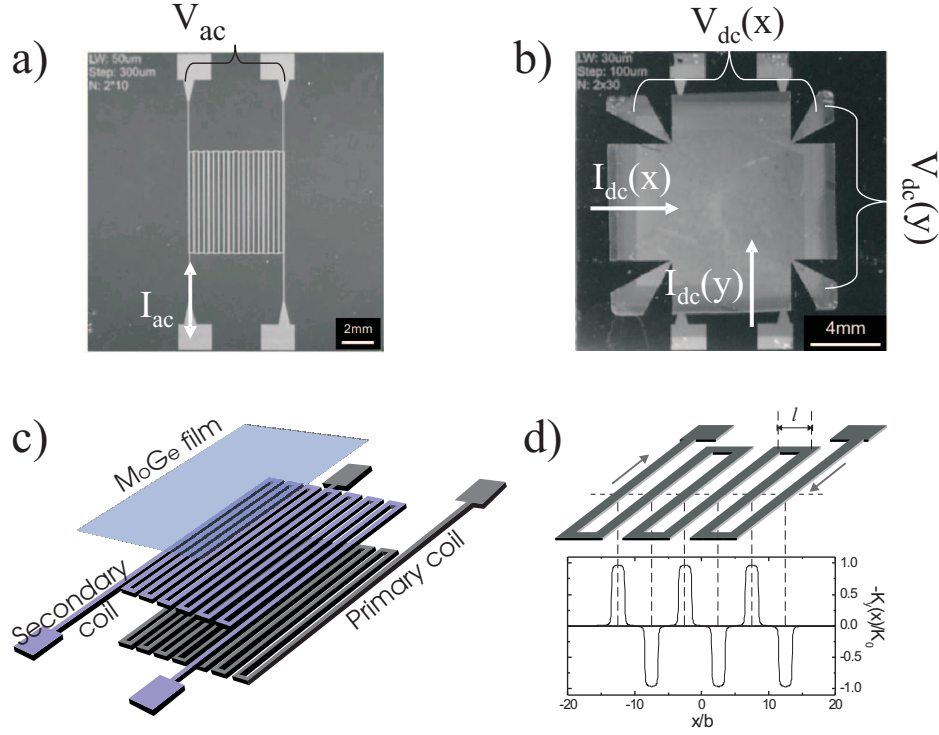
Fig. 1. a. Photograph of the microfabricated Al coils. b. Photograph of the superconducting amorphous film on top of the serpentine coils. Overlapped are indicated the electrical contacts. c. Schematics of the measurement configuration. d. Profile of the current density induced by the primary coil in the sample.
