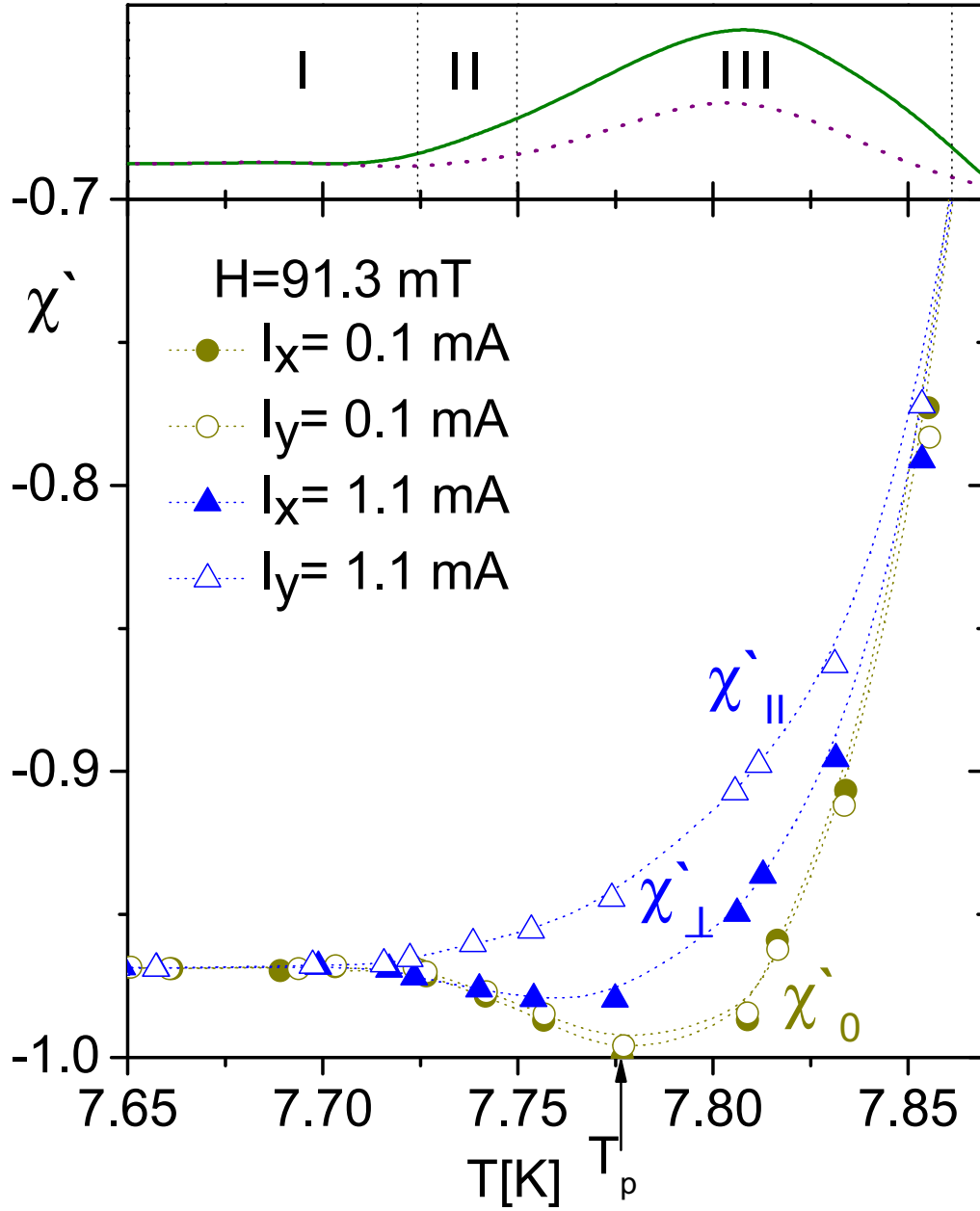
Fig. 2. Bottom panel: Real part of the susceptibility taken with two bias currents in the sample of 0.1 mA and 1.1 mA for one applied magnetic field perpendicular to the film. Open symbols corresponds to the data taken when the bias current on the sample is parallel to the long side of the coils. Closed symbols: bias current perpendicular to the long side of the coils. Dotted lines are splines to the data. Top panel: Subtraction of the \chi_{\parallel} and \chi_{\perp} fits to the reference \chi_0 fit (green and purple line respectively) showing the first three phases found.
