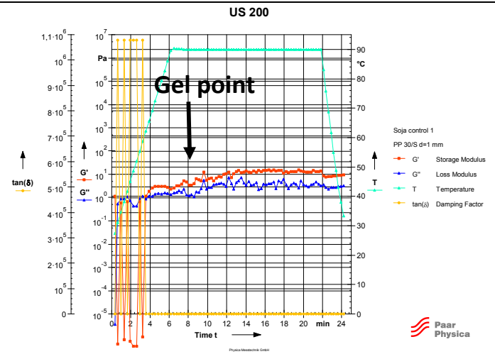
Figure 2. Evolution of storage or elastic components ( G' ), loss or viscous ( G'' ), \tan and temperature ramp, for SPI.
