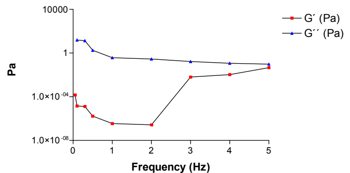
Figure 3. Evolution of solid components ( G' ) and viscose ( G'' ), with frequency for SPI.
