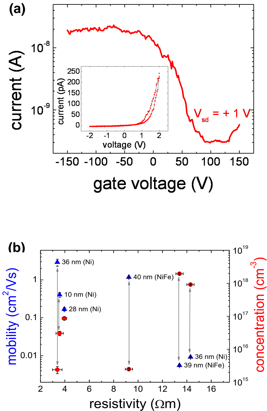
Figure 5. (a) Transfer and current-voltage characteristics of a 28 nm Ni-seeded nanowire showing p-type field-effect switching behavior. In the main figure a current-gate voltage curve taken at 1 V
