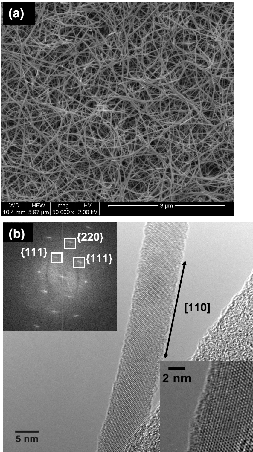
Figure 1. (a) SEM image illustrating the high density 1D Ge nanostructures grown from Ni nanoparticles. The HRTEM image shown in (b) represents a highly crystalline nanowire with a \langle 110 \rangle growth direction (inset in (b) shows the high crystal quality of the nanowires synthesised).
