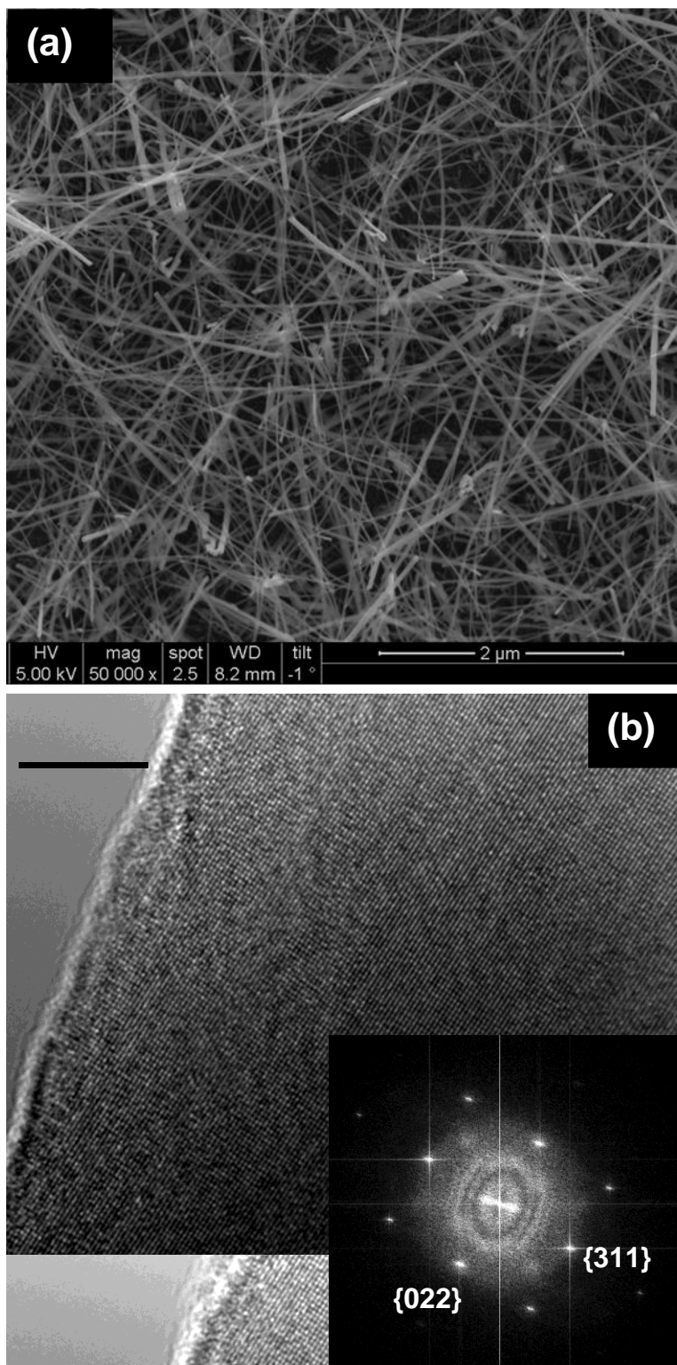
Figure 4. (a) SEM image of Ge nanowires grown from an Ni/Fe alloy coating shows a bimodal diameter distribution. The 1D materials are highly crystalline as shown in the HRTEM in (b) and the corresponding FFT.
