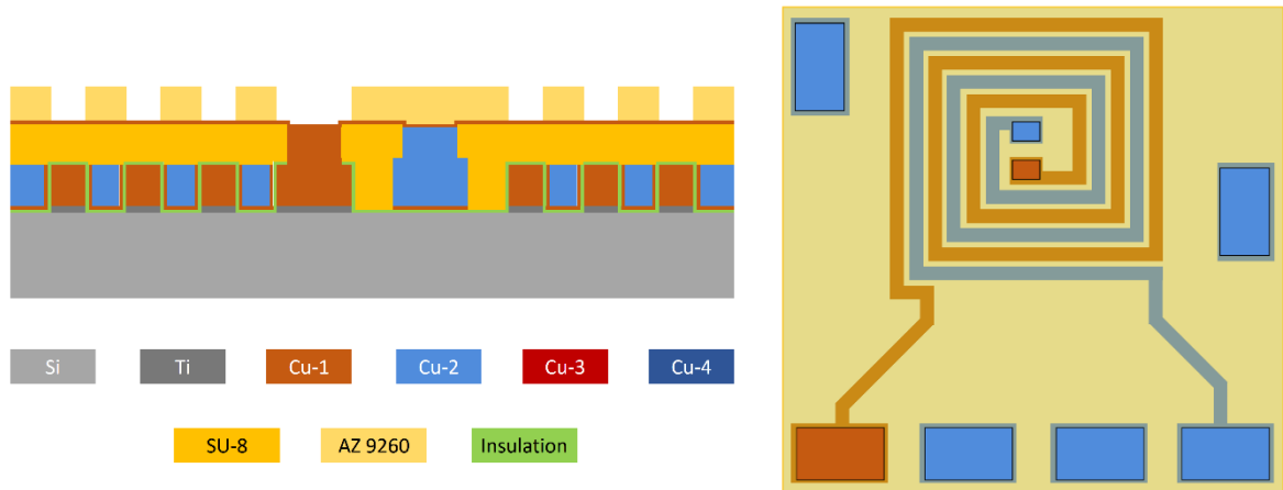
Figure 7.28: Spin-coating of AZ9260 photoresist, and patterning of the coil layer 3.
