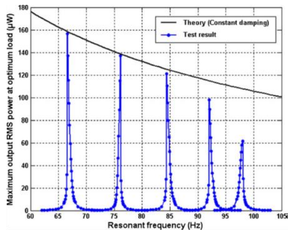
Figure 2.38: (a) Magnetically tunable energy harvester developed by Zhu, et al. [132]. (b) The device is tunable in a range of 67.6 – 98 Hz by variable magnetic force.
