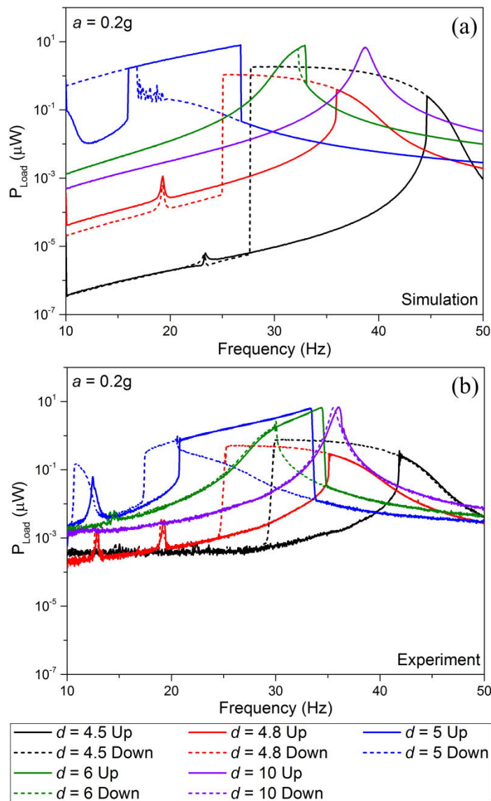
Figure 4.15: (a) Simulated and (b) Experimental frequency sweep responses for different values of d ( a = 0.2\text{g} , R_{\text{Load}} = 1 \text{ k}\Omega ).
