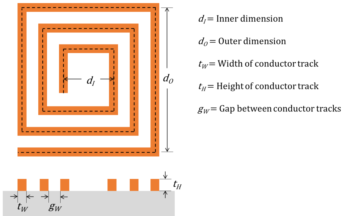
Figure 7.3: Schematic representation of planar square-shaped spiral micro-coil.
