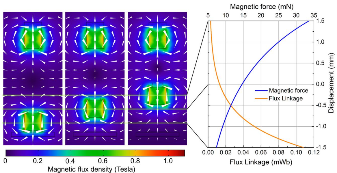
Figure 6.13: Magnetic flux distribution at different positions of the transducing magnet ( z = -1.5 mm, 0 mm, +1.5 mm). Magnetic field directions are denoted by white arrows. The magnetic flux linkage through the coil varies exponentially, while the magnetic force decreases with distance from the coil.
