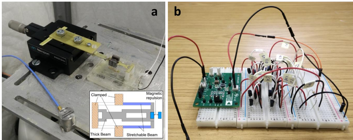
Figure 8.9: (a) Vibration energy harvester mounted on shaker table. Inset shows the device topology. (b) The power management module comprising CRD circuit, DELVD rectifier and ADP5090 board.
