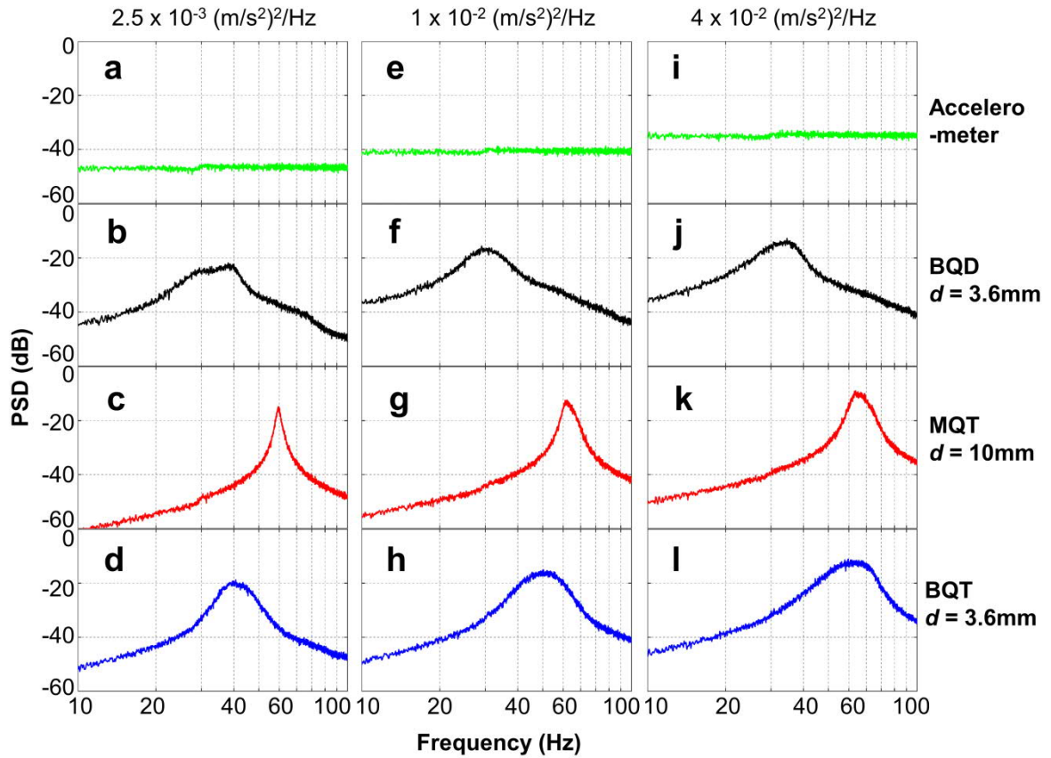
Figure 5.11: Power spectral density (PSD) vs frequency plots for the BQD, MQT and BQT configurations under band limited (10-110 Hz) random vibrations of 2.5 \times 10^{-3} (\text{m/s}^2)^2/\text{Hz} , 1 \times 10^{-2} (\text{m/s}^2)^2/\text{Hz} , and 4 \times 10^{-2} (\text{m/s}^2)^2/\text{Hz} average PSD.
