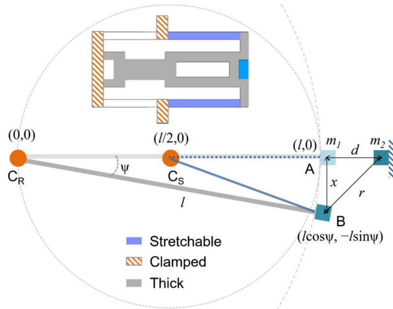
Figure 5.4: Schematic model of the BQT oscillator. The thick, stretchable and clamped sections of the spring structure has been identified.
