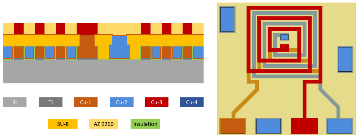
Figure 7.29: Electrodeposition of the coil layer 3, which is connected to coil layer 1 through inter-level via.
