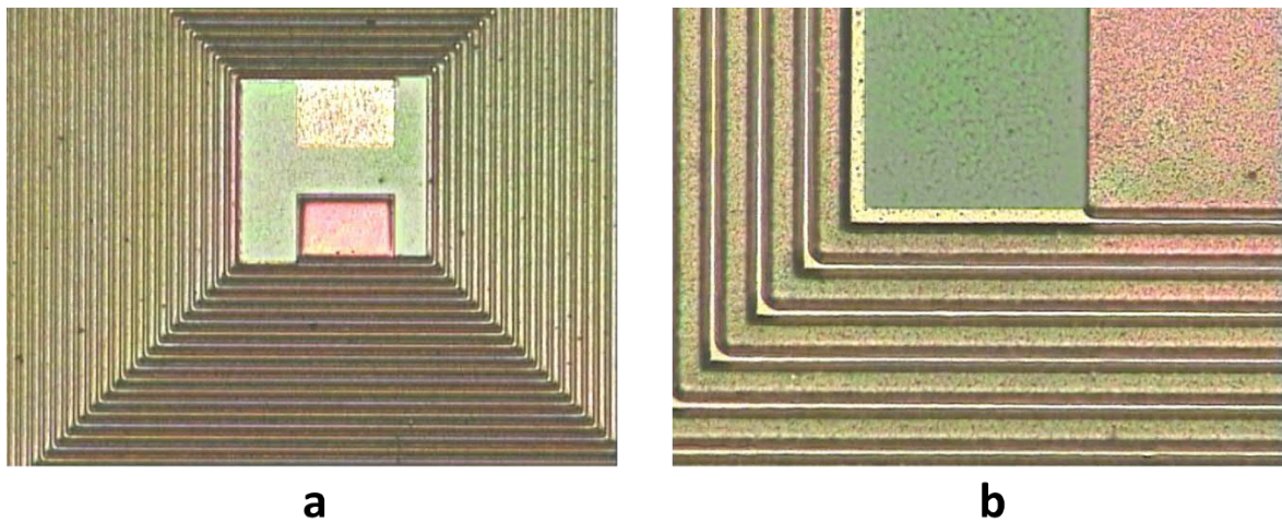
Figure 7.47: (a) Ultra-dense coil with 1 μm thick Parylene C as insulating layer between coil layers 1 and 2. (b) Formation of micro-bubbles in the Parylene C.
