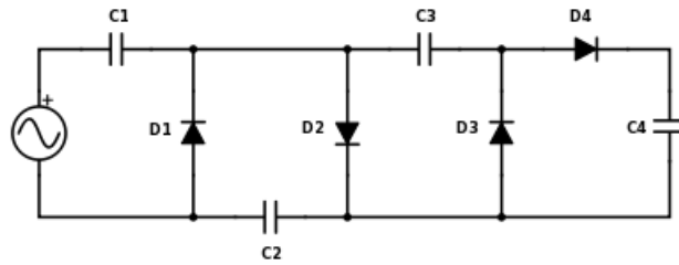
Figure 2.44: Voltage quadrupler circuit with ladder configuration
