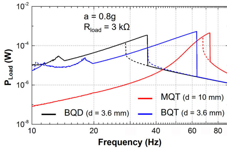
Figure 5.6: Numerically simulated frequency responses for the BQD (bistable-quadratic), MQT (monostable-quartic) and BQT (bistable-quartic) VEHs. The solid and dashed lines represent the forward sweep response and the reverse sweep responses.
