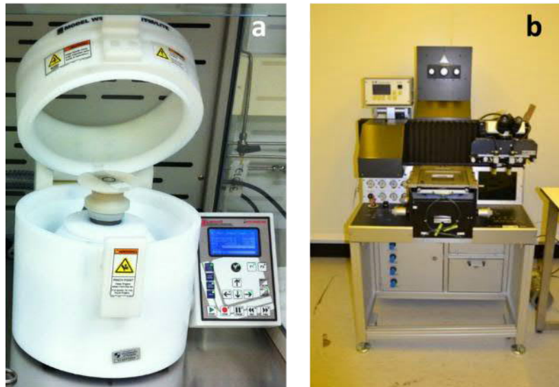
Figure 3.6: (a) Laurell WS 650 spin coater. (b) Karl-Suss MA6 mask aligner.
