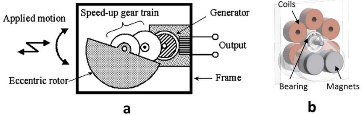
Figure 2.2: Electromagnetic energy harvester after (a) Seiko Instruments Inc. and (b) Spreemann, et al. [3].
