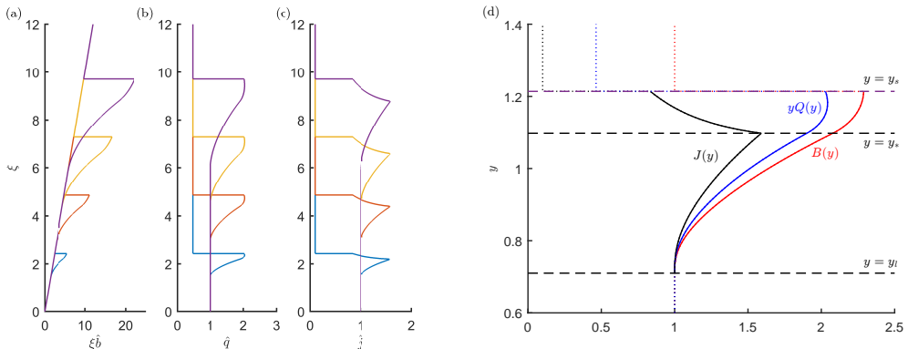
FIGURE 7. (a)-(c) The rescaled width \xi\hat{b}(\xi) , volume flux, \hat{q}(\xi) and buoyancy flux, \hat{j}(\xi) as functions of the dimensionless distance from source, \xi , for an instantaneous increase in the buoyancy flux per unit width at the origin ( \mathcal{F} = 0.1 ) at dimensionless times \tau = 2, 4, 6 & 8. (d) The similarity solution for B(y) , Q(y) and J(y) as functions of the similarity variable, y (solid lines) and the results from the direct numerical integration of the governing equations (3.2) (dotted lines). Note that the two solutions are virtually indistinguishable. Also shown are three important locations ( y_l, y_{si}, y_s ) in the construction of the similarity solution. In these computations, S = 1.2 and S_f = 1.2 .
