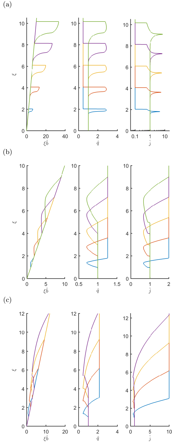
FIGURE 4. The rescaled width \xi \hat{b}(\xi) , volume flux, \hat{q}(\xi) and buoyancy flux, \hat{j}(\xi) as functions of the dimensionless distance from source, \xi , for various ratios of the source buoyancy flux, \mathcal{F} imposed upon the system at \tau = 0 . (a) \mathcal{F} = 0.1 and \tau = 2, 4, 6, 8, 10 ; (b) \mathcal{F} = 2 and \tau = 2, 4, 6, 8, 10 ; and (c) \mathcal{F} = 10 and \tau = 1, 2, 3, 4 ; In all computations, S = 1.1 and S_f = 1 .
