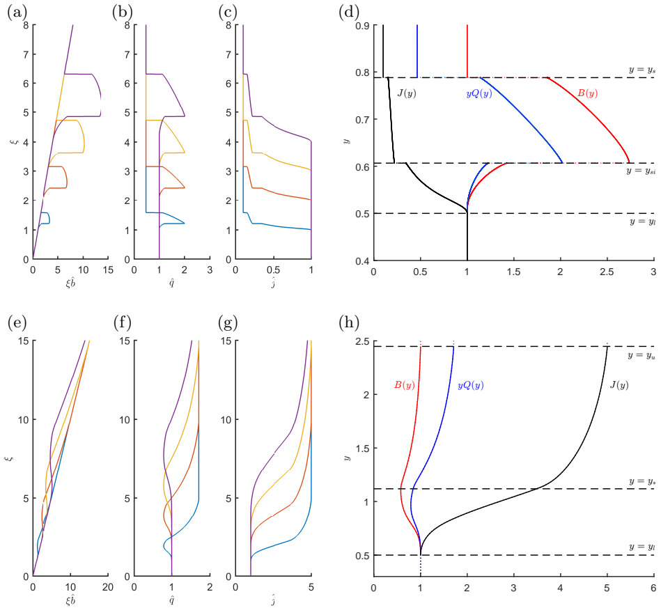
FIGURE 10. (a)-(c),(e)-(g) The rescaled width \xi \hat{b}(\xi) , volume flux, \hat{q}(\xi) and buoyancy flux, \hat{j}(\xi) as functions of the dimensionless distance from source, \xi , at dimensionless times \tau = 2, 4, 6 & 8 for (a)-(c) an instantaneous increase in the buoyancy flux per unit width at the origin ( \mathcal{F} = 0.1 ); and (e)-(g) an instantaneous decrease in the buoyancy flux per unit width at the origin ( \mathcal{F} = 5 ). (d,h) The similarity solutions for B(y) , Q(y) and J(y) as functions of the similarity variable, y (solid lines) and the results from the direct numerical integration of the governing equations (3.2) (dotted lines) for (d) \mathcal{F} = 0.1 and (h) \mathcal{F} = 5 . Note that the similarity solution and the direct numerical integration are virtually indistinguishable. Also shown are important locations in the construction of the similarity solution: (d) (y_l, y_{si}, y_s) and (h) (y_l, y_*, y_u) . In these computations, S = 1.1 and S_f = 0.5 .
