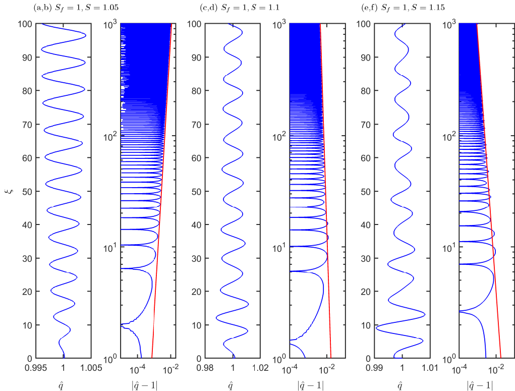
FIGURE 2. The rescaled volume flux per unit width, \hat{q}(\xi, \tau) , as a function of dimensionless distance from source, \xi , for the perturbed boundary condition \mathbf{q}(0, \tau) = (1, 1, 1 + \epsilon e^{i\tau}) and various values of the shape factor, S , while S_f = 1 in each case: (a), (b) \tau = 790 and S = 1.05 ; (c), (d) \tau = 699 and S = 1.1 ; and (e), (f) \tau = 640 and S = 1.15 . Also plotted in (b), (d) & (f) are the theoretically predicted growth/decay rates.
