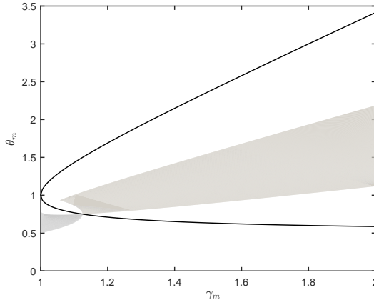
FIGURE 9. The regions of the plane of shape factors, (\gamma_m, \theta_m) , for which the steady line plume solution (C.1) is linearly stable to harmonic disturbances to the source (shaded region, corresponding to \sigma_i < 0 , i = 1-3 ). Also plotted are the parameter values for which the governing system of equations is ill-posed (solid lines)
