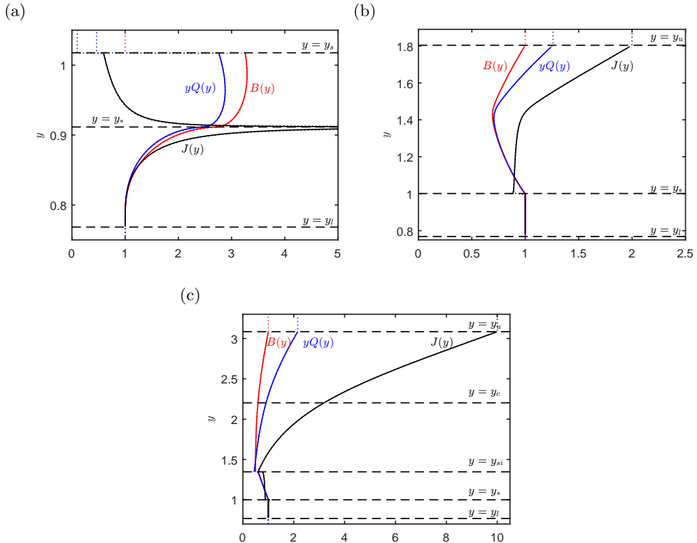
FIGURE 5. (a–c) The similarity solutions for the width, B(y) , volume flux, yQ(y) , and buoyancy flux, J(y) = y^3 G(y)Q(y)/B(y) = \hat{j} , for a line plume in response to an instantaneous change in source strength as functions of the similarity variable y (solid lines) and their evaluation from direct numerical integration of (3.2) (dotted lines) for (a) \mathcal{F} = 10 ; (b) \mathcal{F} = 0.5 ; (c) \mathcal{F} = 0.1 . In this case S = 1.1 and S_f = 1 . Also plotted are various important locations within the solution ( y_l , y_* , y_{si} , y_c , y_s and y_u ). Note that the similarity solution and numerical integration are virtually indistinguishable.
