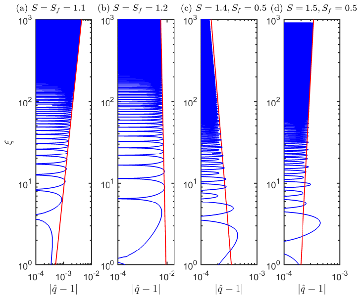
FIGURE 3. The rescaled flux per unit width, \hat{q}(\xi, \tau) , as a function of dimensionless distance from source, \xi , for the perturbed boundary condition \mathbf{q}(0, \tau) = (1, 1, 1 + \epsilon e^{i\tau}) and various values of the shape factors: (a) \tau = 700 and S = S_f = 1.1 ; (b) \tau = 592 and S = S_f = 1.2 ; (c) \tau = 620 , S = 1.4 and S_f = 0.5 ; and (d) \tau = 1450 , S = 1.5 and S_f = 0.5 . Also plotted in (a)-(d) are the theoretically predicted growth/decay rates.
