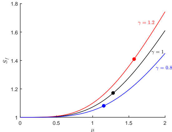
FIGURE 8. The shape factor, S_f , as a function of the scaled width parameter, \mu , for various ratios \gamma (see (A 25)). Also plotted are the parameter values, (\mu, S_f) , for each value of \gamma at which the line plume equations first become linearly stable to harmonic disturbances at the source to their steady state.
