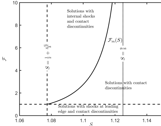
FIGURE 6. The regimes of similarity solutions in the (S, \mathcal{F}) plane for S_f = 1 . Also plotted is the buoyancy flux ratio at source, at which internal shocks first appear, \mathcal{F}_m , as a function of the shape factor S (solid line). The value S = 1/2 + \sqrt{3}/3 is plotted (dashed line) and this corresponds to the threshold for linearly stable solutions, while solutions with internal shocks are not found for S > 9/8 .
