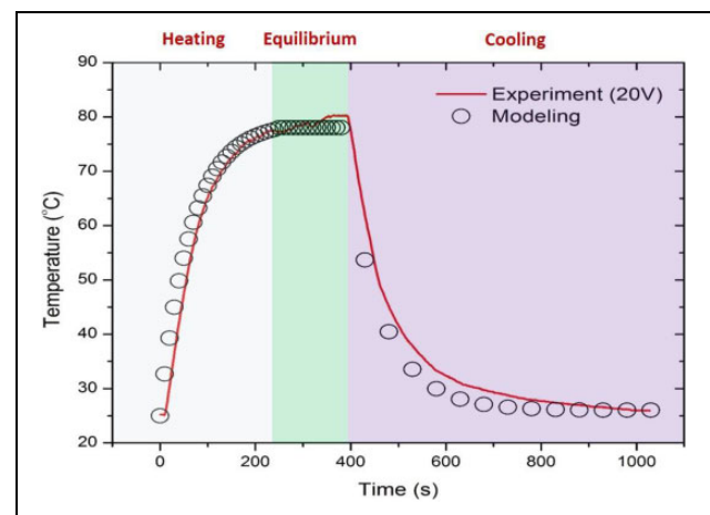
Figure 8. Analytical modeling for heating performance of CNT/PDMS composite films. CNT: carbon nanotube; PDMS: polydimethylsiloxane.
