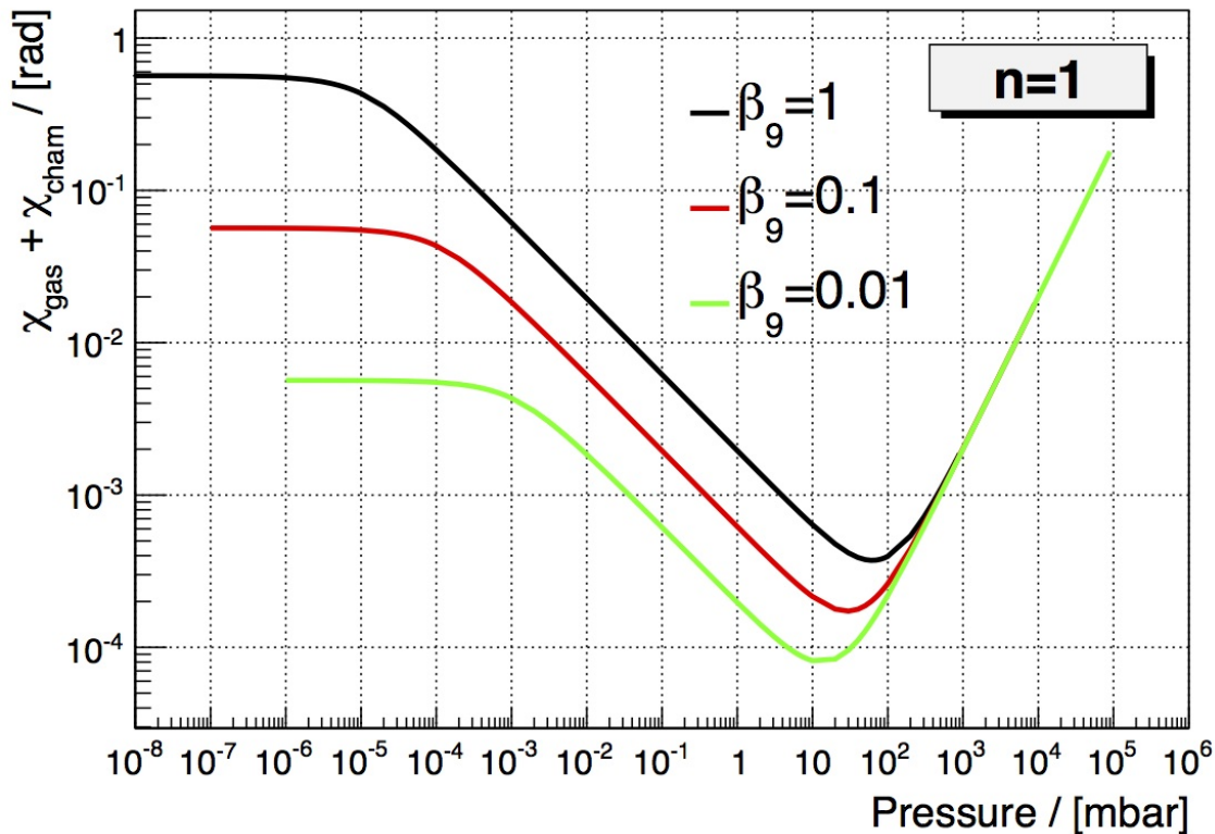
Figure 2. Calculation of the sum of the chameleon and gas mixture phase shifts for the conditions described in the text as a function of the gas pressure. The linear term at high pressure comes from the phase shift due to the neutron optical potential of the gas. The yellow line for \beta_m of 1 \times 10^7 sets the sensitivity goal for the experiment.
