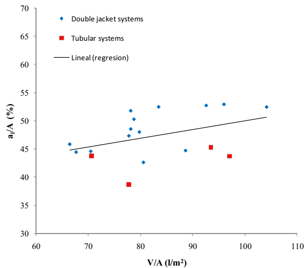
Fig. 2: a_1/A vs V/A
