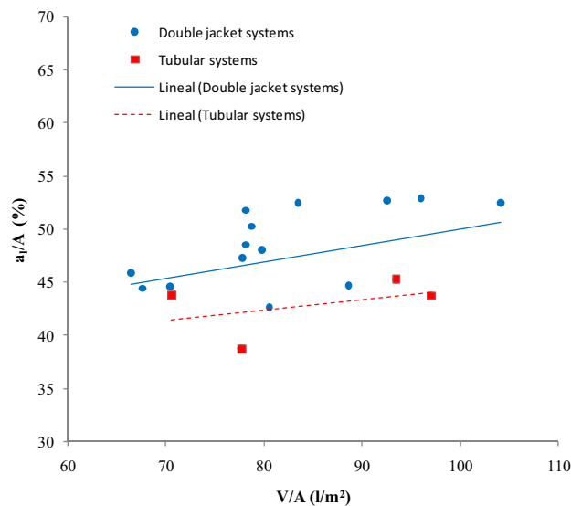
Fig. 3: a_1/A vs V/A
