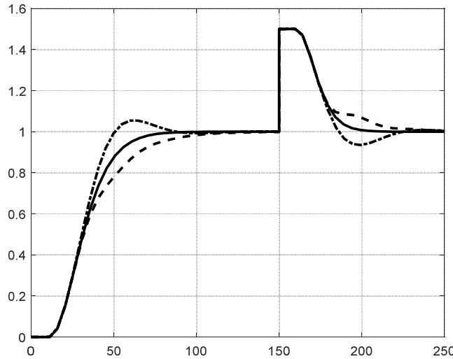
Figure 8. Step response of the control system with the YOULA controller.
